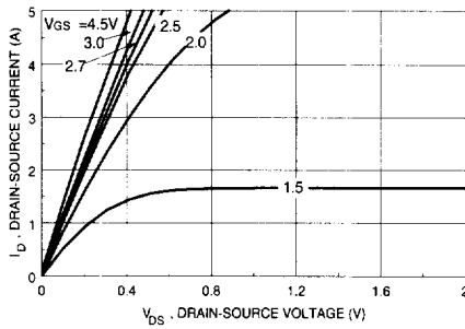
Figure 1. On-Region Characteristics.
