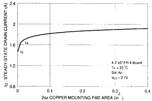
Figure 16. Maximum Steady-State Drain Current versus Copper Mounting Pad Area.
