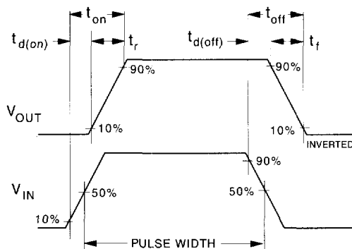
Figure 12. Switching Waveforms.
