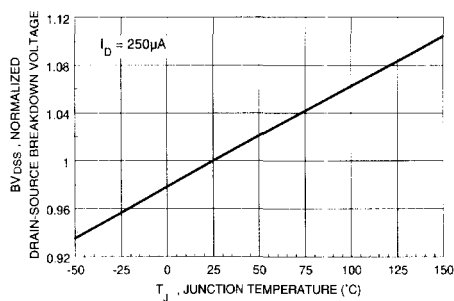
Figure 7. Breakdown Voltage Variation with Temperature.
