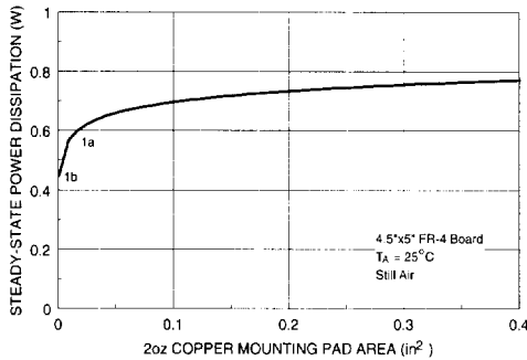
Figure 15. SuperSOT™-3 Maximum Steady-State Power Dissipation versus Copper Mounting Pad Area.
