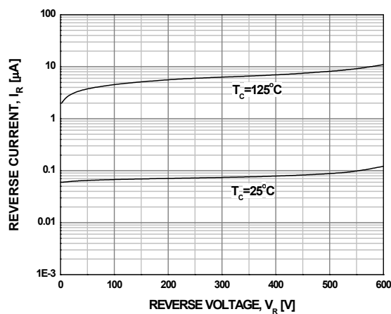
Figure 4. Typical Reverse Current
