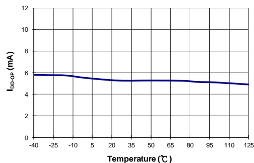
Figure 10. Operating Current
