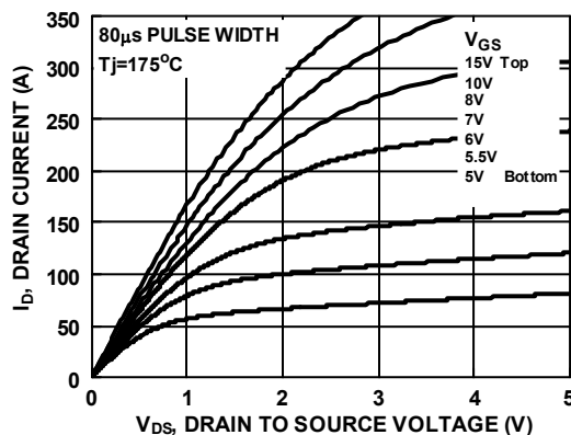
Figure 10. Saturation Characteristics
