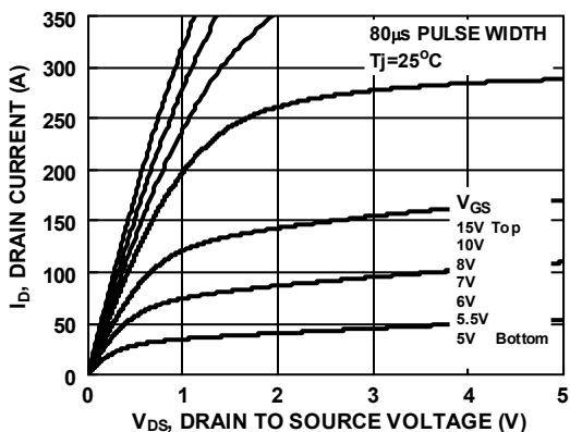
Figure 9. Saturation Characteristics
