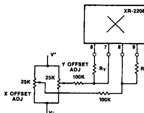
Figure 13. Offset Adjustment
