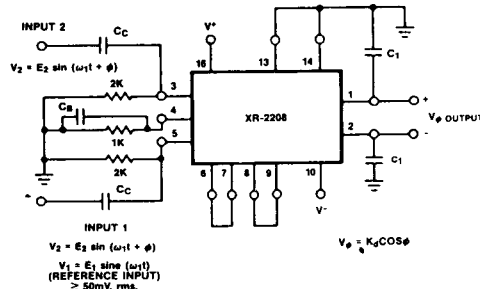
Figure 20. Phase-Detector Circuit
