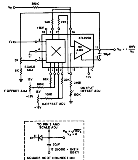
Figure 16. Dividing Circuit
