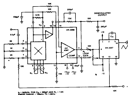
Figure 23. Precision PLL
