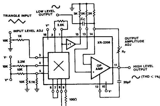
Figure 19. Triangle-to-Sine Converter
