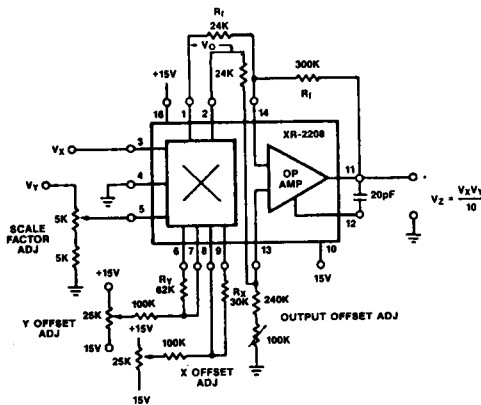
Figure 14. Multiplication Circuit
