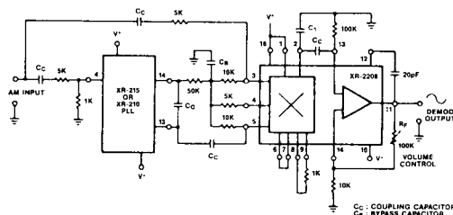
Figure 24. Phase-Locked AM Demodulation or Carrier Detection
