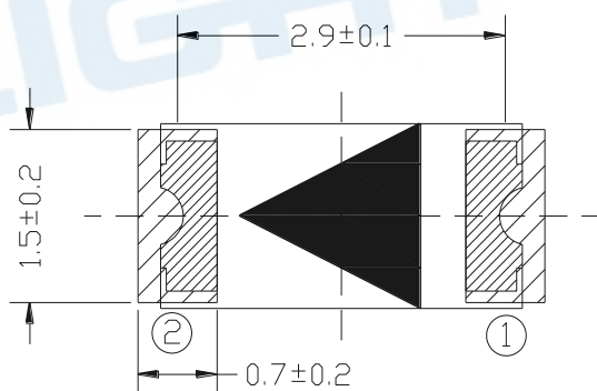
Recommend Soldering Pad
