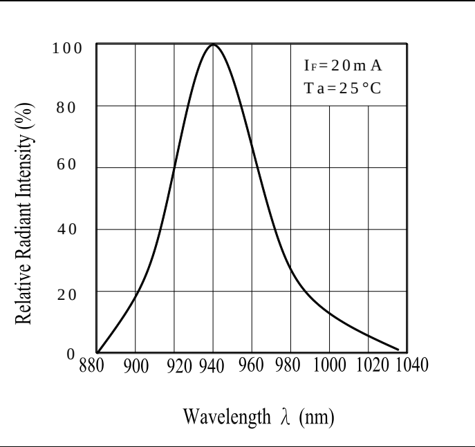
Spectral Sensitivity
