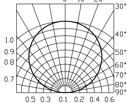
Radiation Diagram
