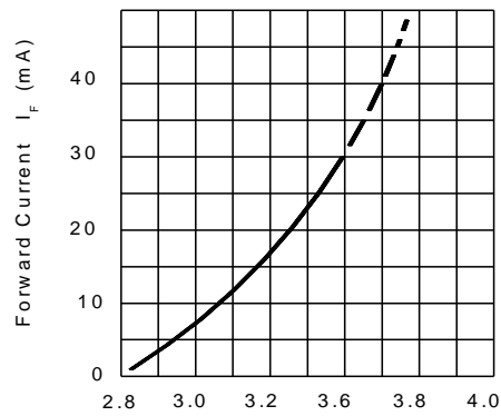
Forward Voltage (V_F) -volts
