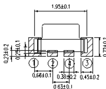
Recommend Soldering Pad
