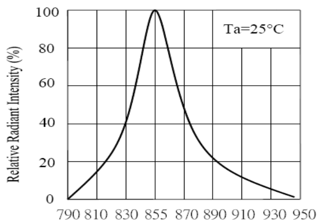
Fig.4 Spectral Distribution
