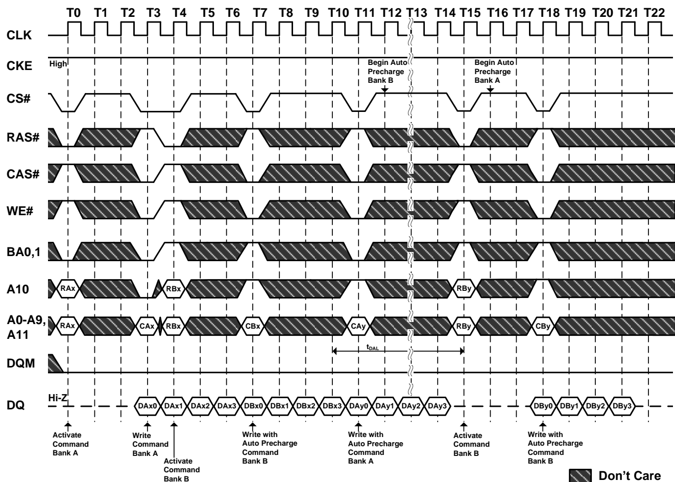
Figure 36. Auto Precharge after Write Burst (Burst Length=4)
