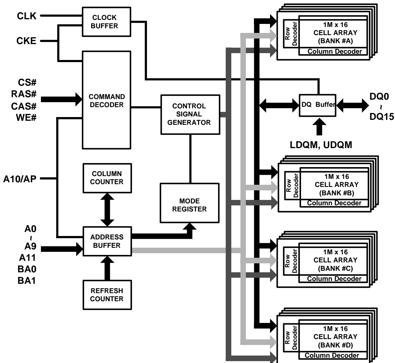
Figure 3. Block Diagram
