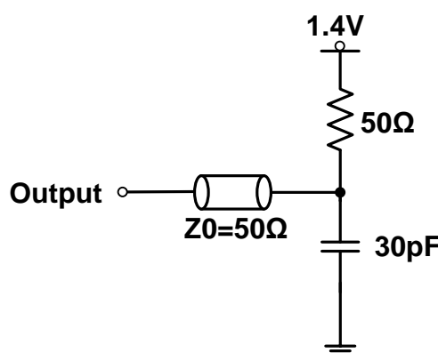
Figure 19.2 LVTTL A.C. Test Load (B)
