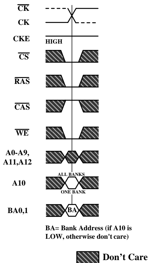
Figure 27. Precharge Command
