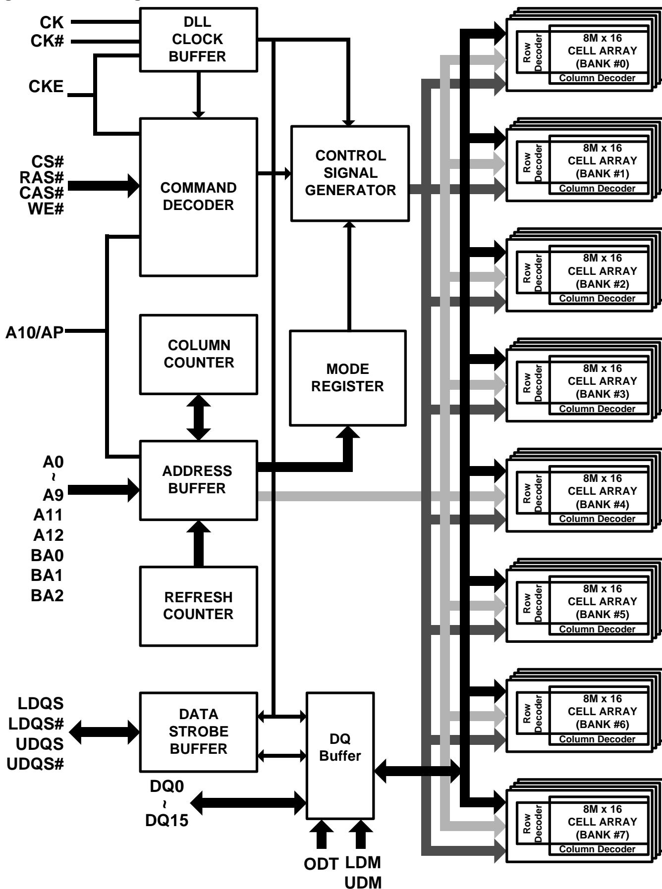
Figure 2. Block Diagram
