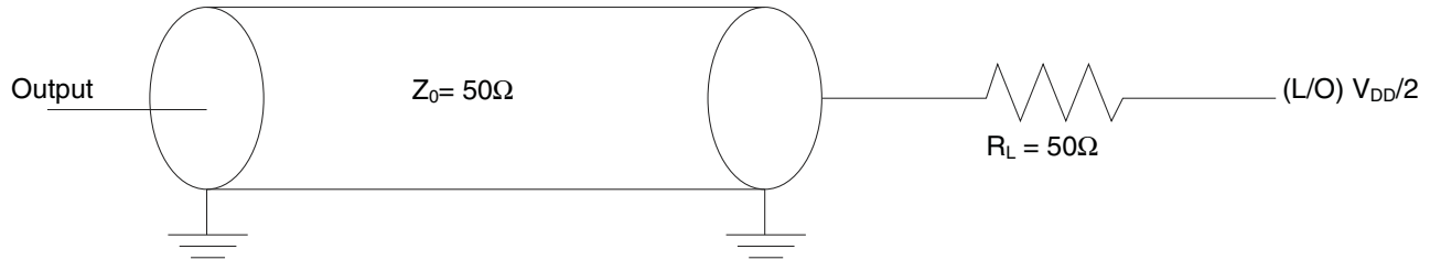
Figure 3-52. GPIO AC test load
