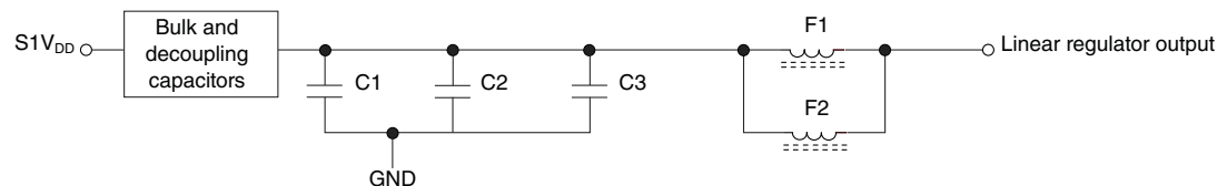
Figure 4-5. SV_{DD} power supply filter circuit
