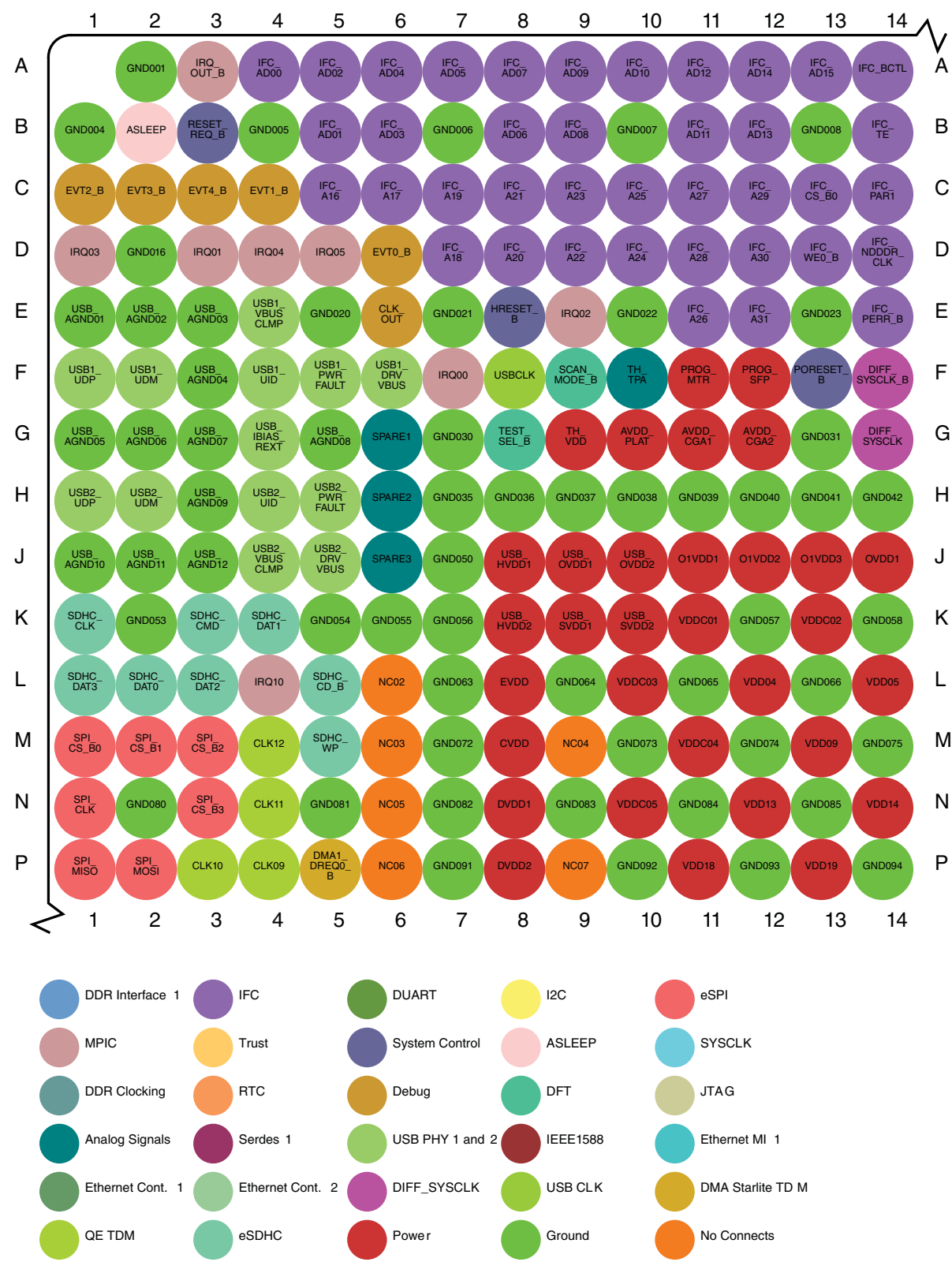
Figure 2-2. Detail A
