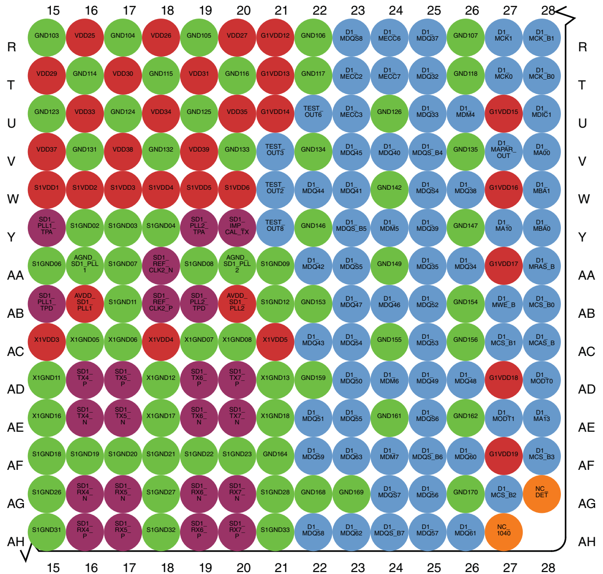
Figure 2-5. Detail D
