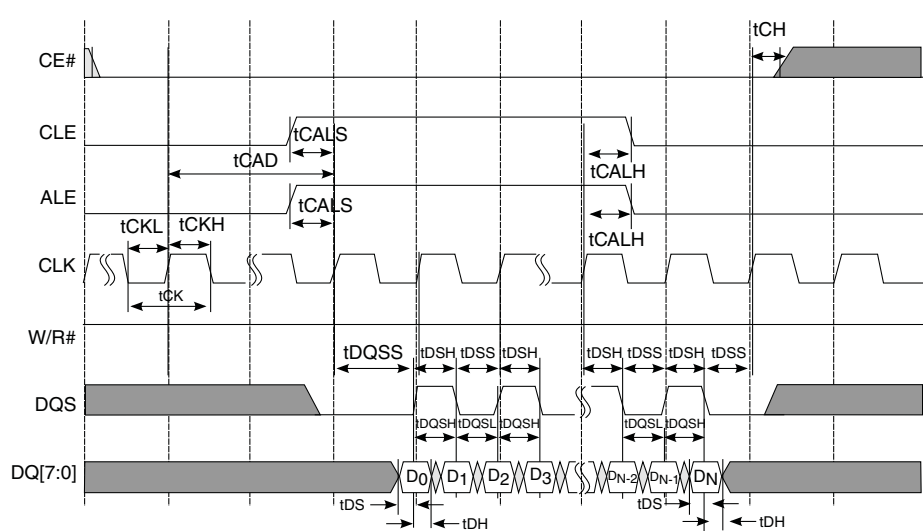
Figure 3-36. Write Cycle
