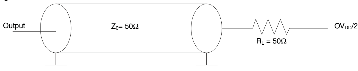
Figure 3-46. AC test load for the JTAG interface
