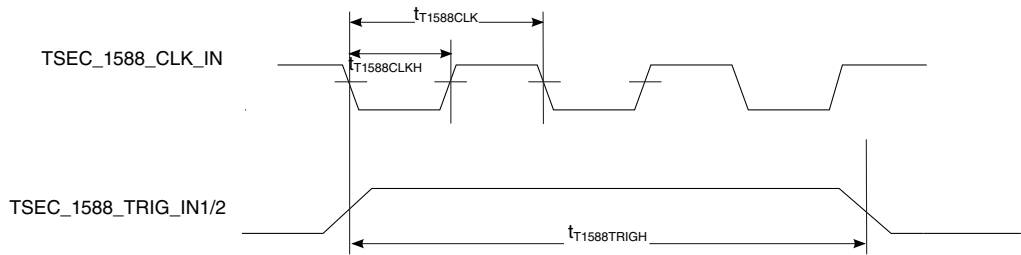
Figure 3-21. IEEE 1588 input AC timing
