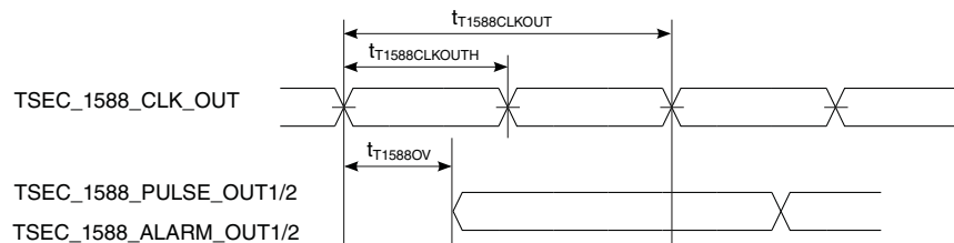
Figure 3-20. IEEE 1588 output AC timing
