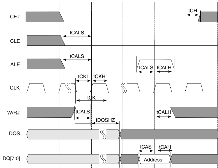
Figure 3-35. Address Cycle
