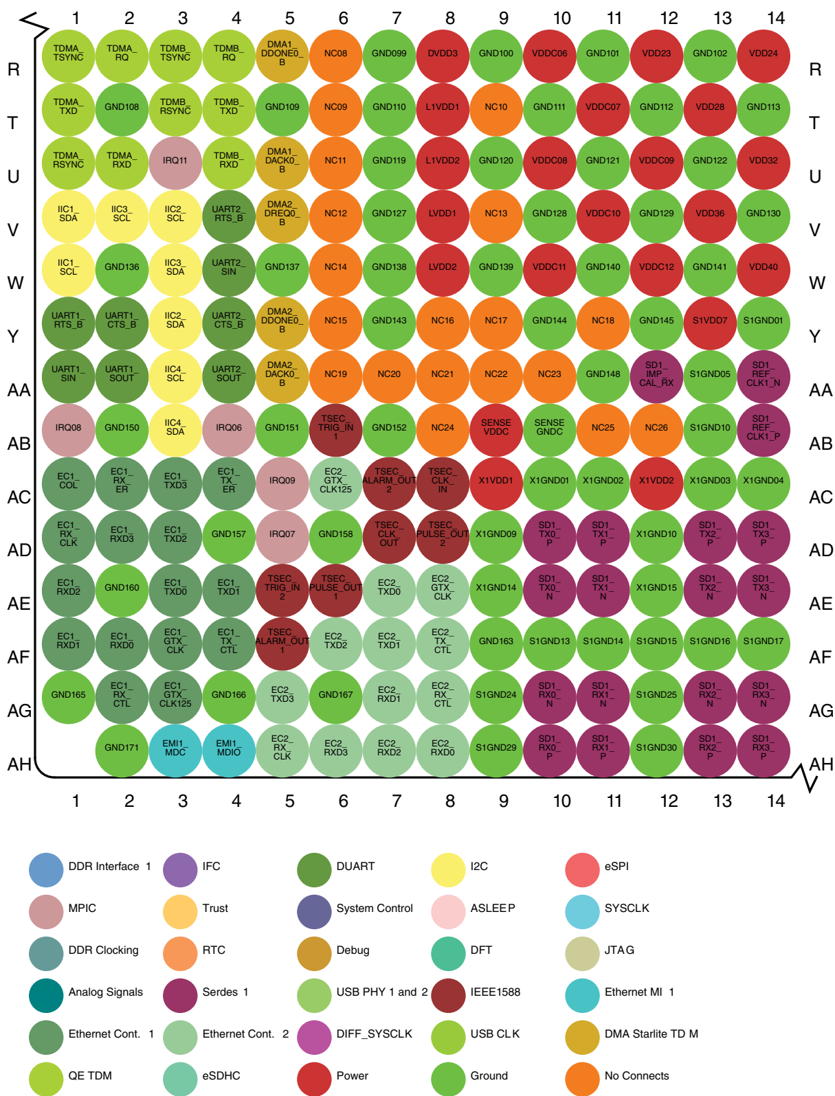
Figure 2-4. Detail C
