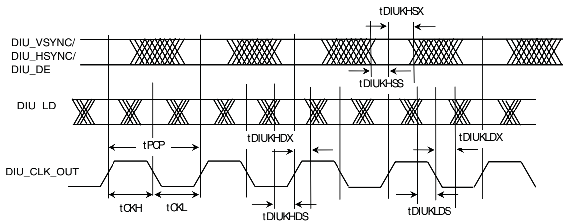
Figure 3-53. DIU interface AC timing diagram
