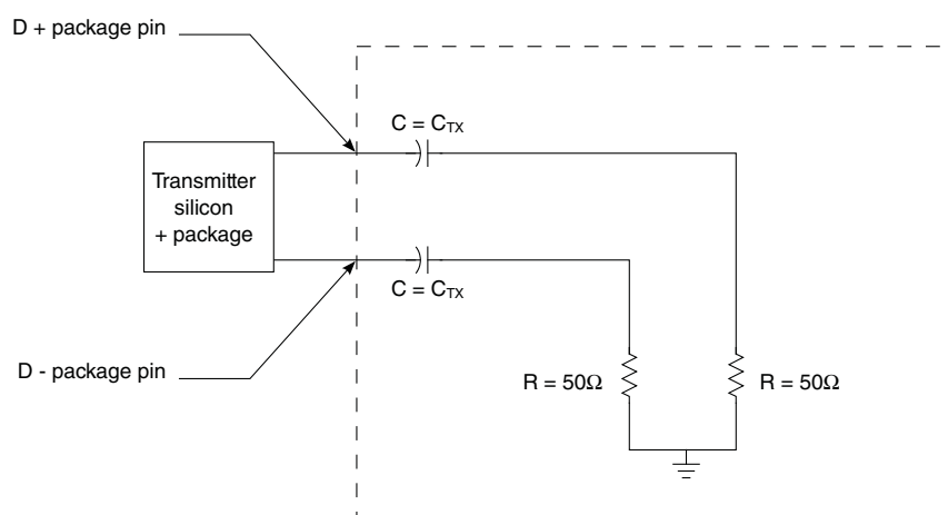
Figure 3-65. Test/measurement load
