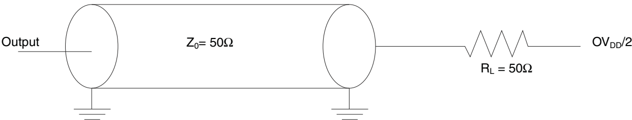
Figure 3-27. Integrated flash controller AC test load
