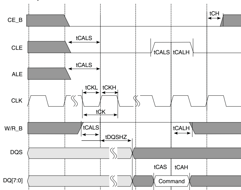
Figure 3-34. Command Cycle
