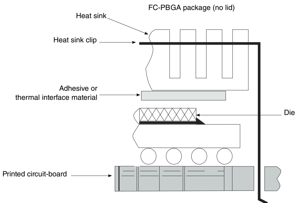
Figure 4-16. Package exploded, cross-sectional view-FC-PBGA (no lid)
