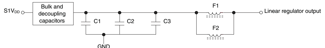
Figure 4-5. SVDD power supply filter circuit
