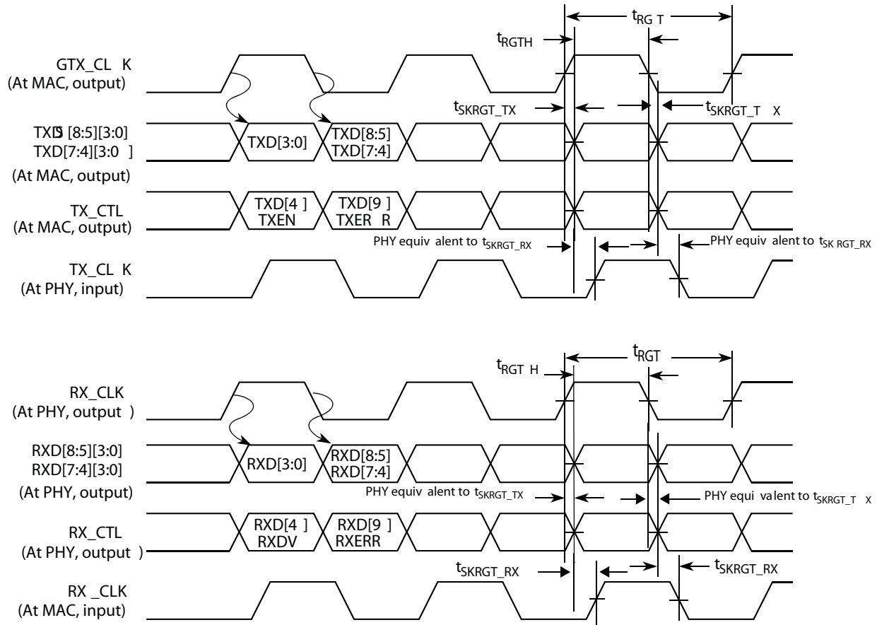
Figure 3-15. RGMII AC timing and multiplexing diagrams
