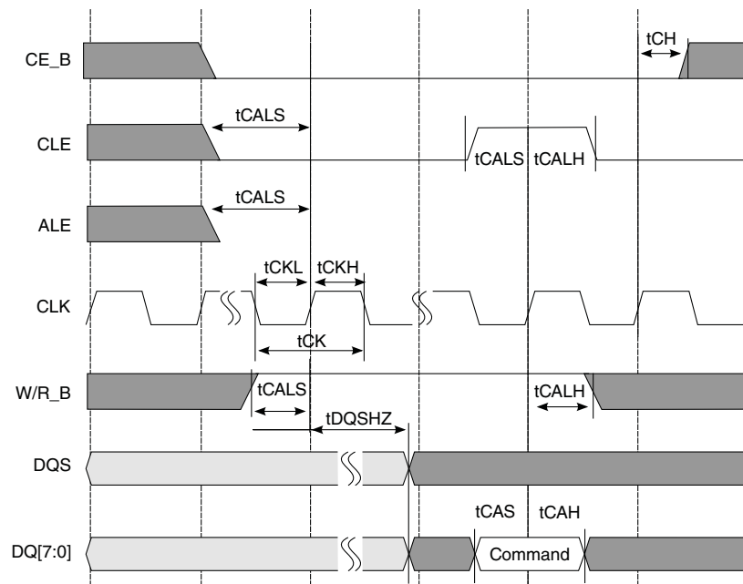
Figure 3-33. Command Cycle
