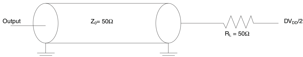
Figure 3-49. 2 C AC test load
