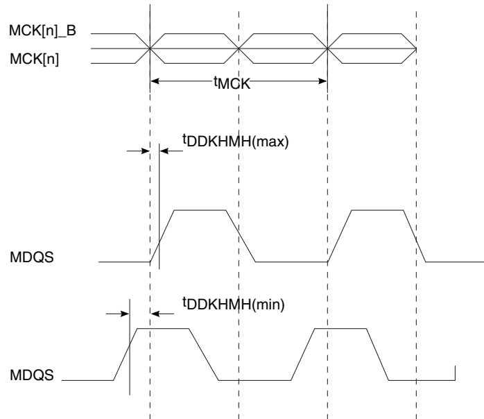
Figure 3-6. t_{DDKMH} timing diagram
