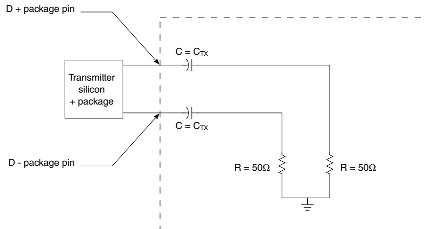
Figure 3-64. Test/measurement load
