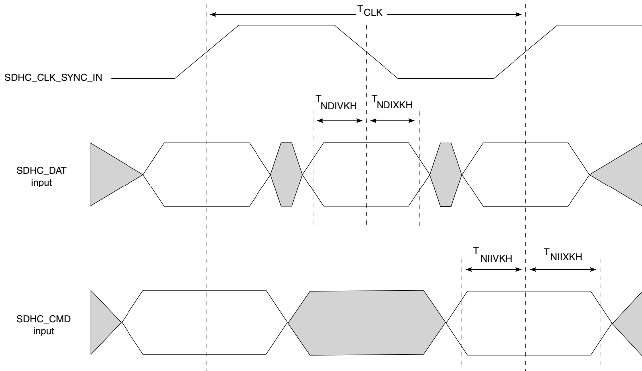
Figure 3-42. eSDHC DDR50/DDR mode input AC timing diagram
