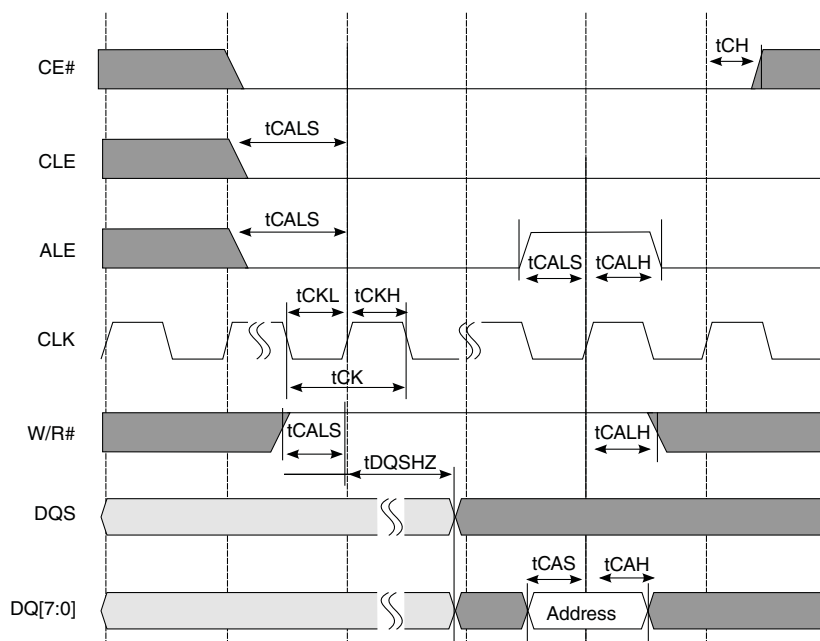
Figure 3-34. Address Cycle
