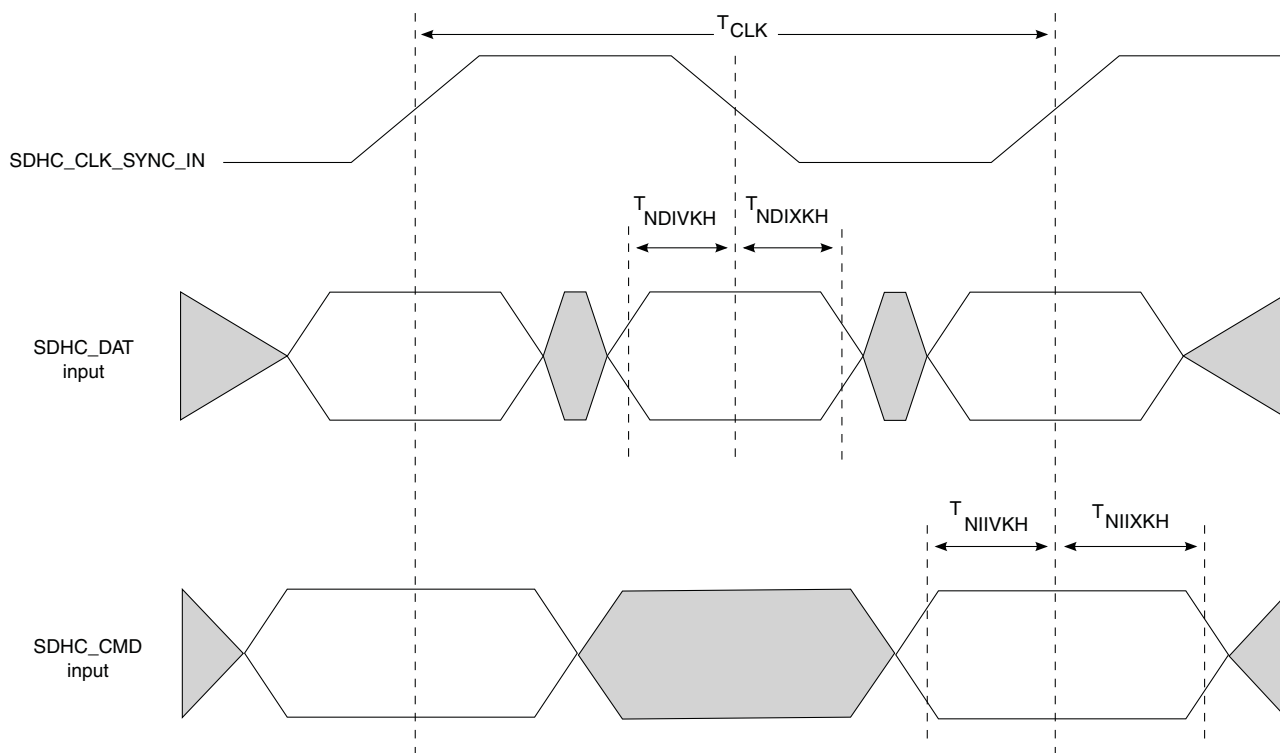
Figure 3-40. eSDHC SDR50 mode input AC timing diagram
