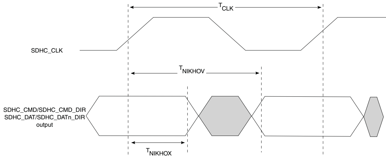
Figure 3-41. eSDHC SDR50 mode output AC timing diagram
