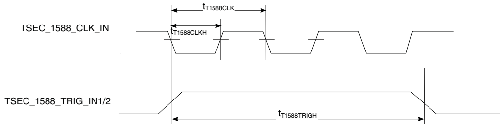
Figure 3-20. IEEE 1588 input AC timing
