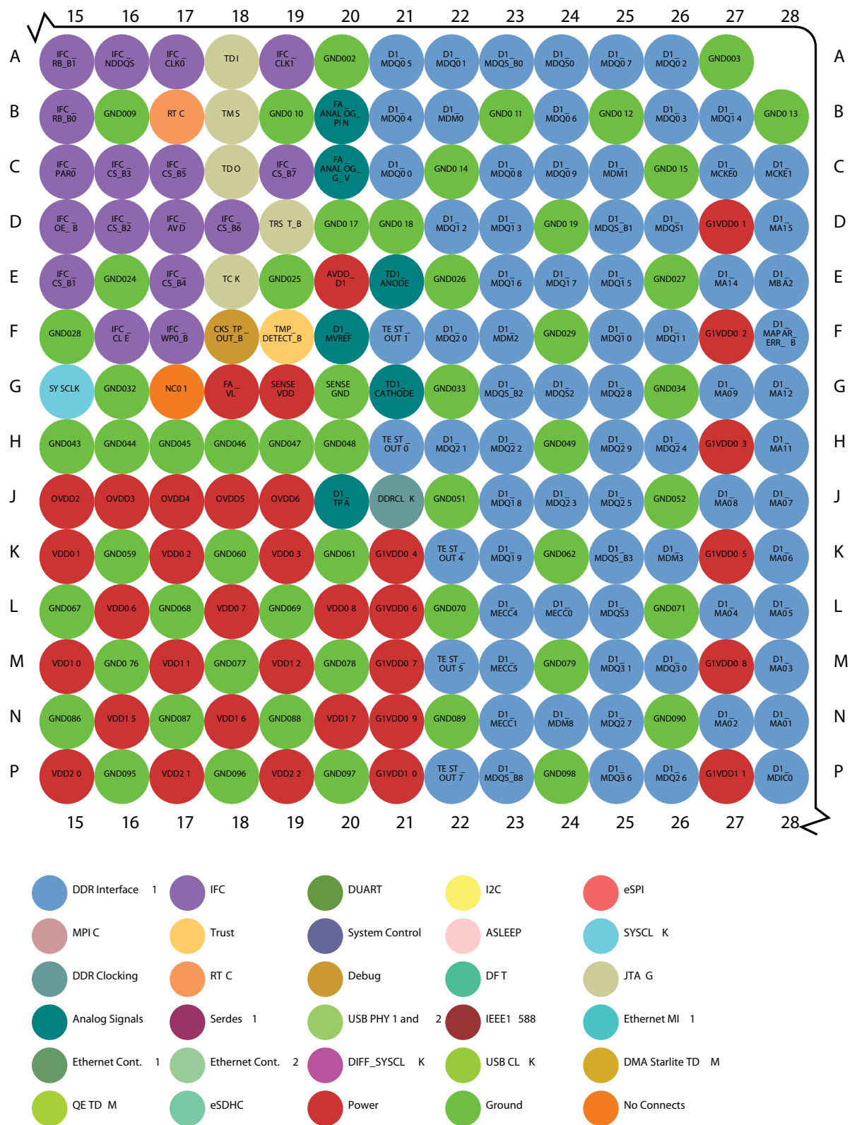
Figure 2-3. Detail B
