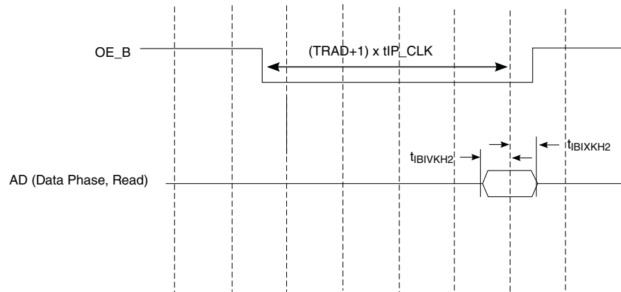
Figure 3-28. IFC-NOR Interface input AC timings
