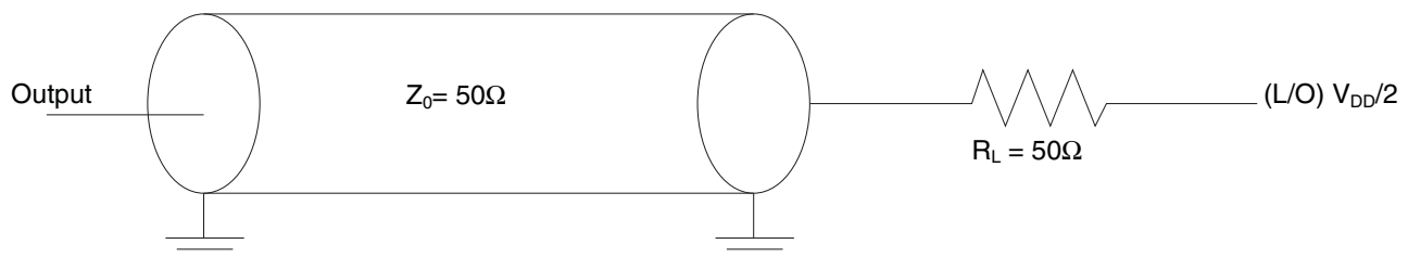
Figure 3-51. GPIO AC test load
