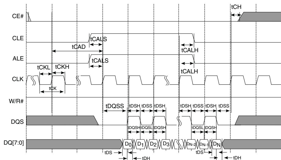
Figure 3-35. Write Cycle
