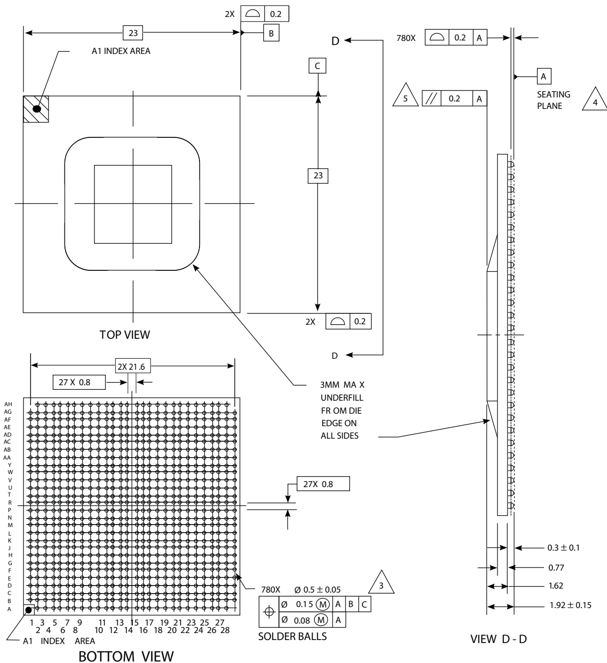
Figure 5-2. Mechanical dimensions of the FC-PBGA - C5 leaded
