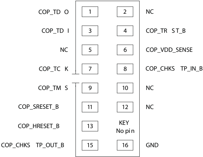
Figure 4-9. Legacy COP Connector Physical Pinout
