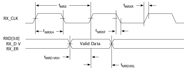
Figure 3-18. MII receive AC timing diagram
