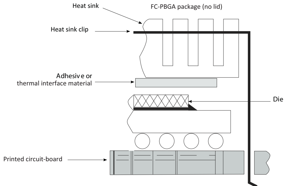
Figure 4-16. Package exploded, cross-sectional view-FC-PBGA (no lid)
