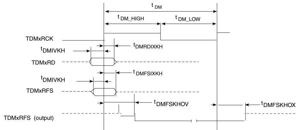
Figure 3-53. TDM Receive Signals
