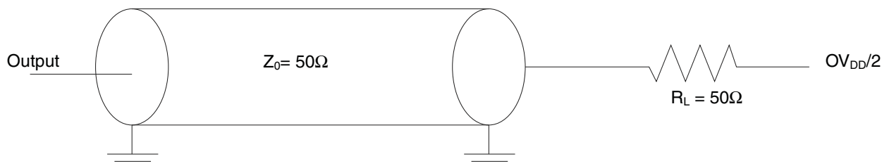
Figure 3-26. Integrated flash controller AC test load
