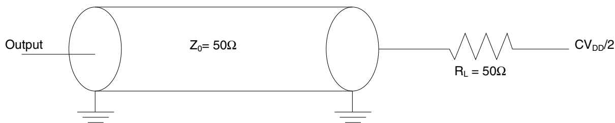
Figure 3-8. eSPI AC test load
