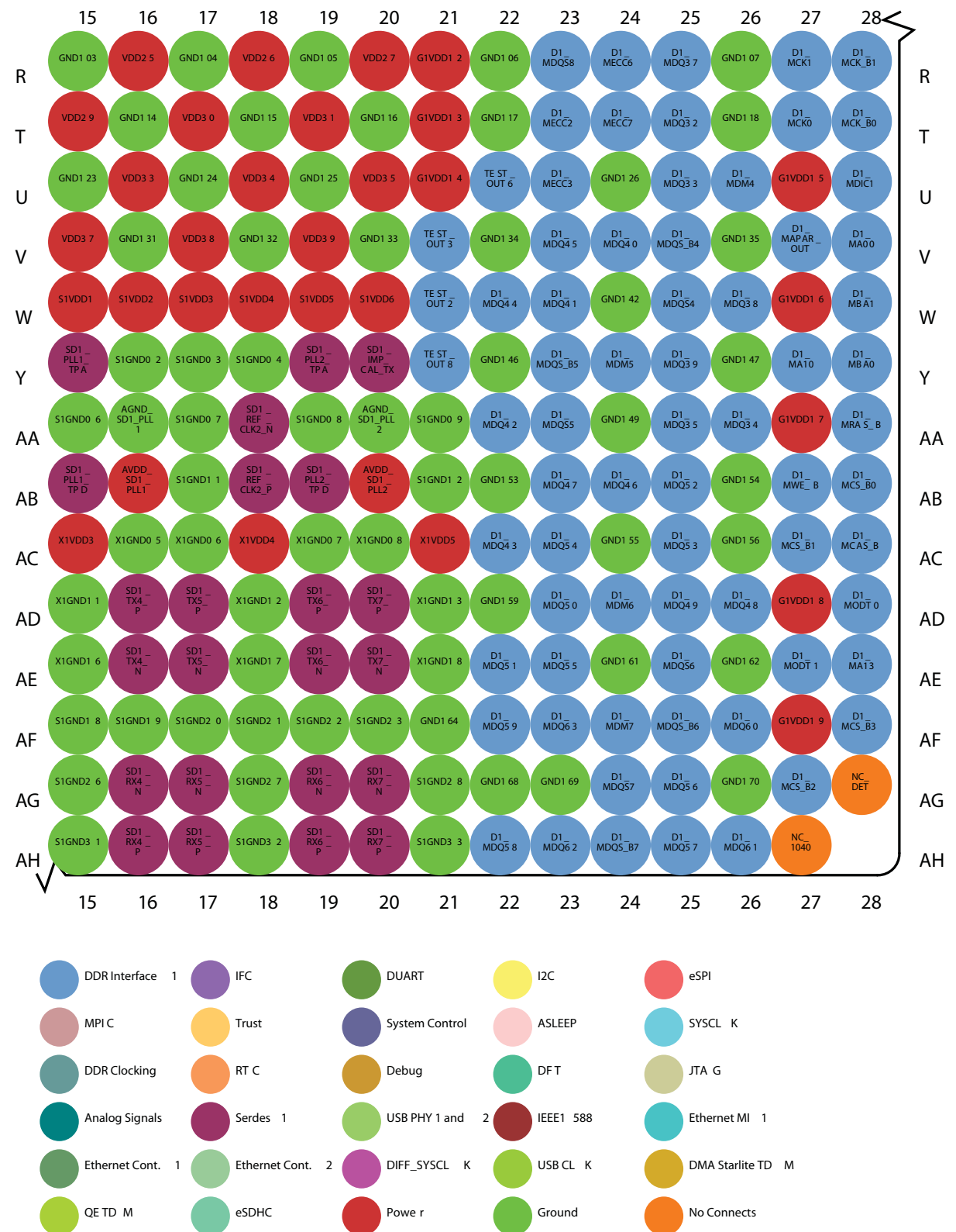
Figure 2-5. Detail D
