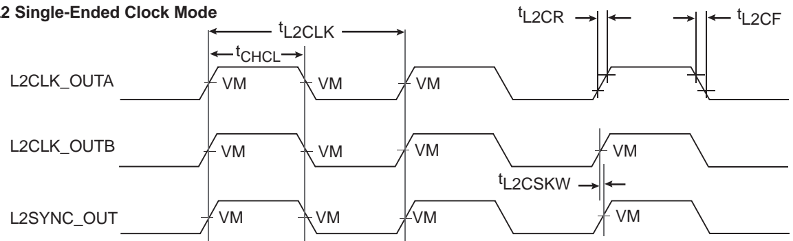
Figure 5-6. L2CLK_OUT Output Timing Diagram
