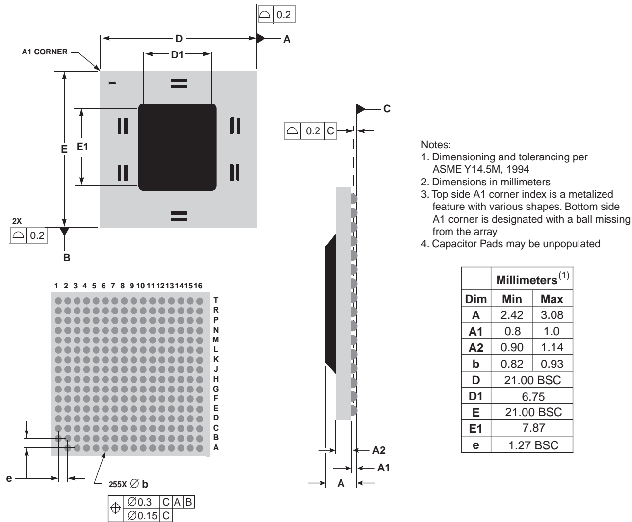
Figure 8-1. Mechanical Dimensions and Bottom Surface Nomenclature of the PC745 HiTCE (GH)
