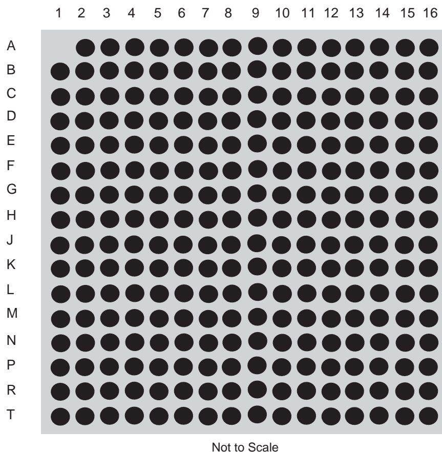
Figure 6-1. Pinout of the PC745, 255 PBGA and HiTCE CBGA Packages as Viewed from the Top Surface
