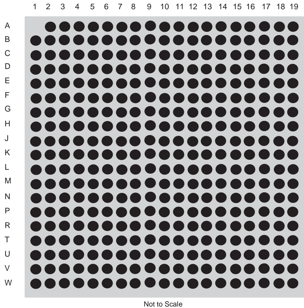
Figure 6-2. Pinout of the PC755, 360 PBGA, CBGA and HiTCE packages as Viewed from the Top Surface Part A
