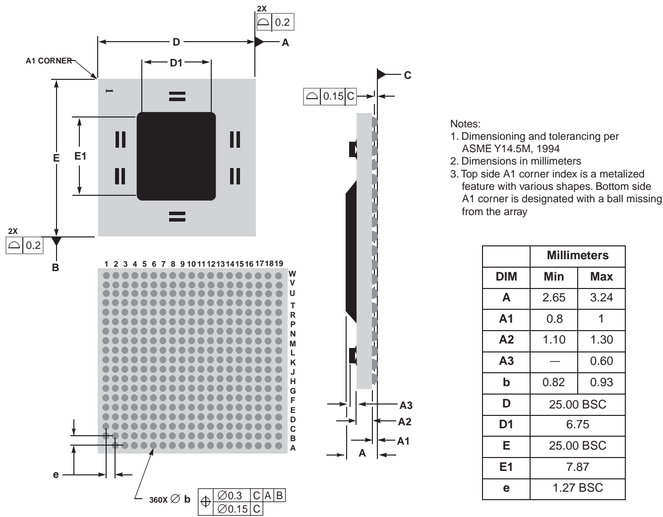
Figure 8-8. Mechanical Dimensions and Bottom Surface Nomenclature of PC755 (HiTCE) (GH)
