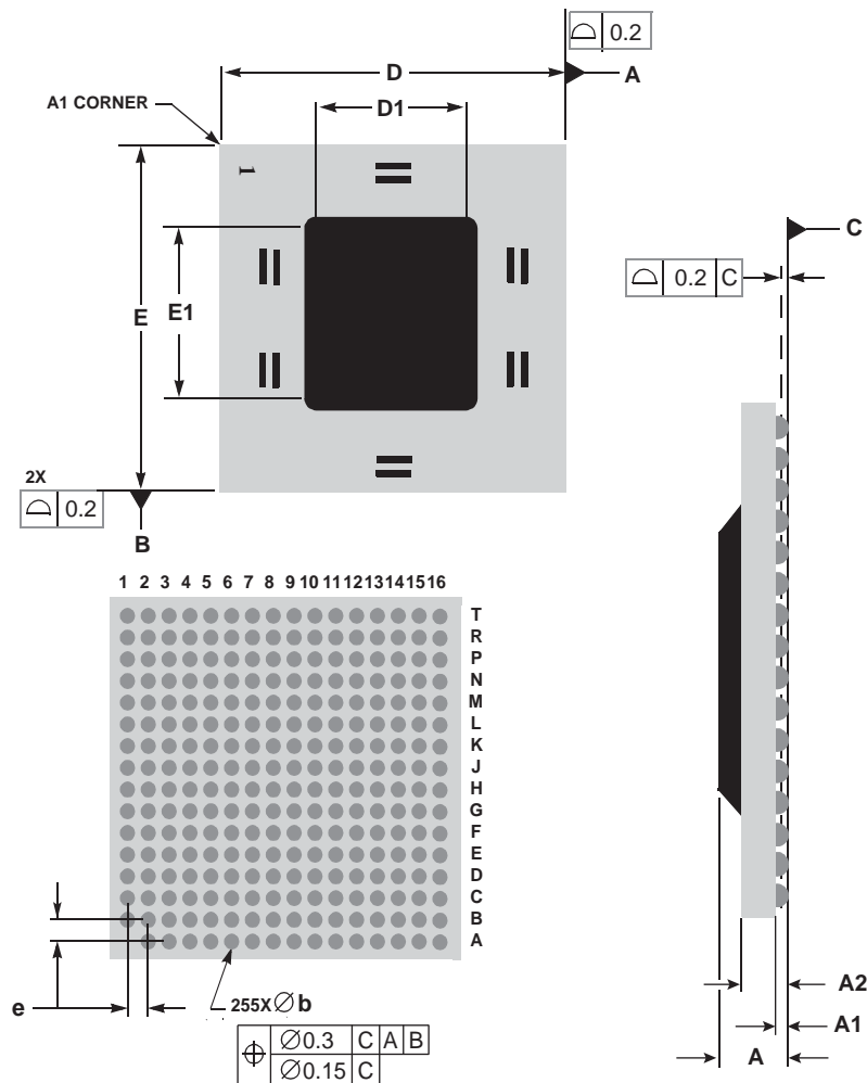
Figure 8-4. Mechanical Dimensions and Bottom Surface Nomenclature of the PC745 (PBGA-RoHS) (ZT)
