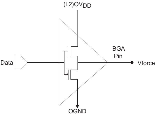
Figure 9-3. Alternate Driver Impedance Measurement Circuit
