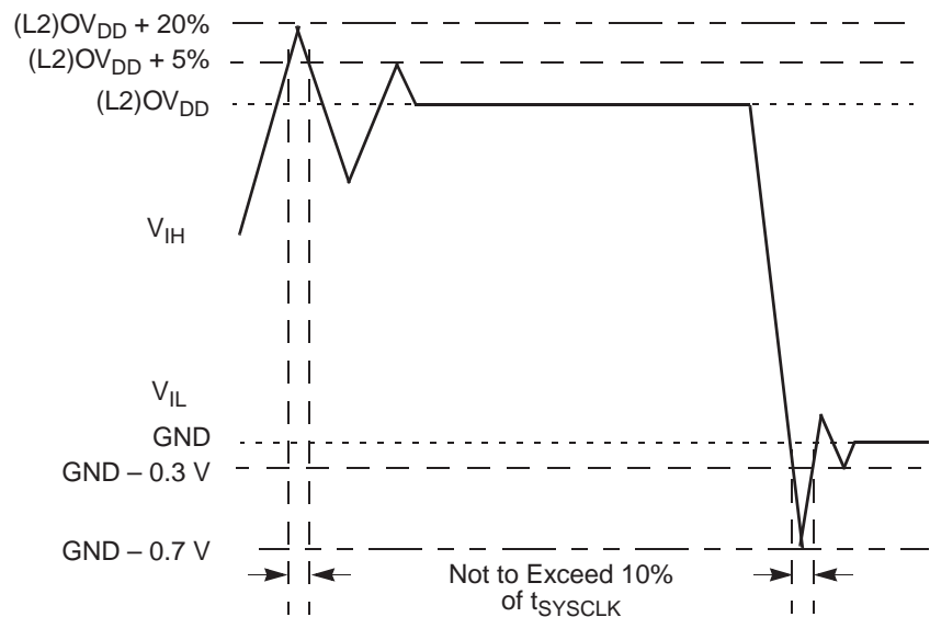
Figure 5-1. Overshoot/Undershoot Voltage
