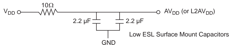
Figure 9-1. PLL Power Supply Filter Circuit
