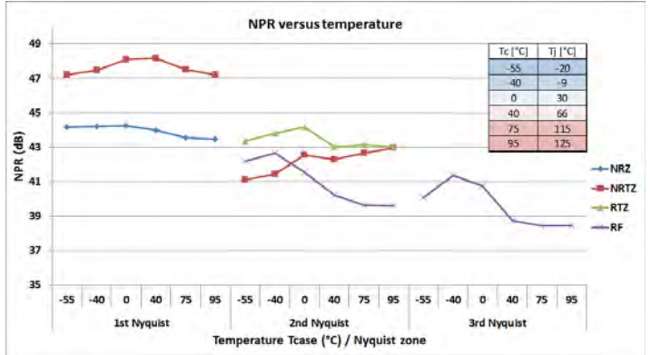
Figure 7-43. NPR versus temperature at 4.5Gps in 4:1MUX, for the four output modes from T_c = -55^{\circ}\text{C} to T_c = 95^{\circ}\text{C} ( T_j = -20^{\circ}\text{C} to 125^{\circ}\text{C} )
