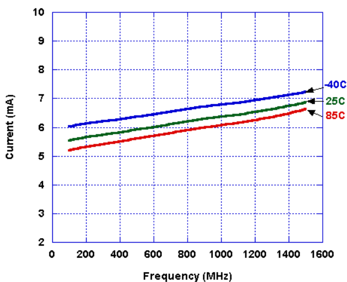
Figure 5. Device Current
