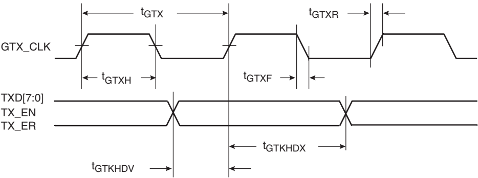
Figure 8-1. GMII Transmit AC Timing Diagram
