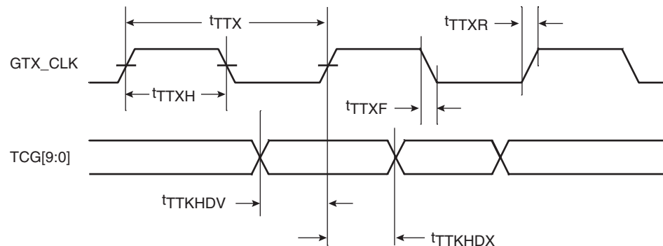
Figure 8-6. TBI Transmit AC Timing Diagram
