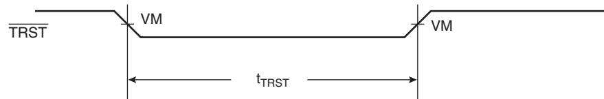
Figure 10-3. \overline{TRST} Timing Diagram
