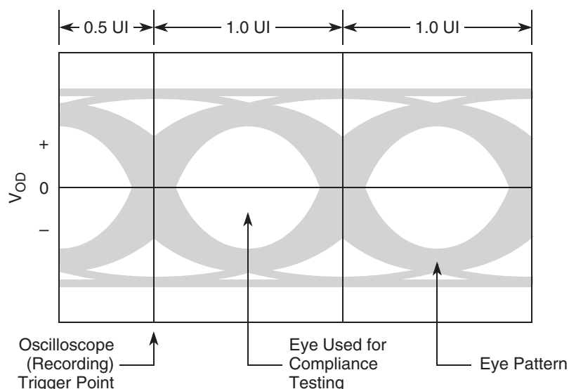
Figure 13-5. Example Driver Output Eye Pattern
