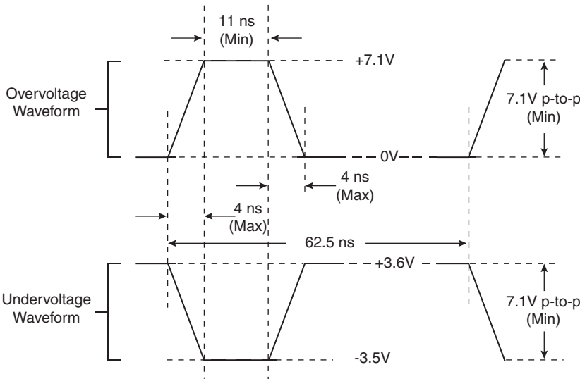
Figure 2-2. Maximum AC Waveforms on PCI Interface for 3.3V Signaling
