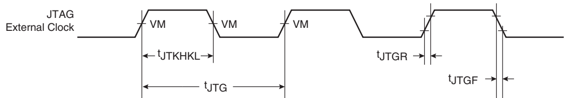
Figure 10-2. JTAG Clock Input Timing Diagram
