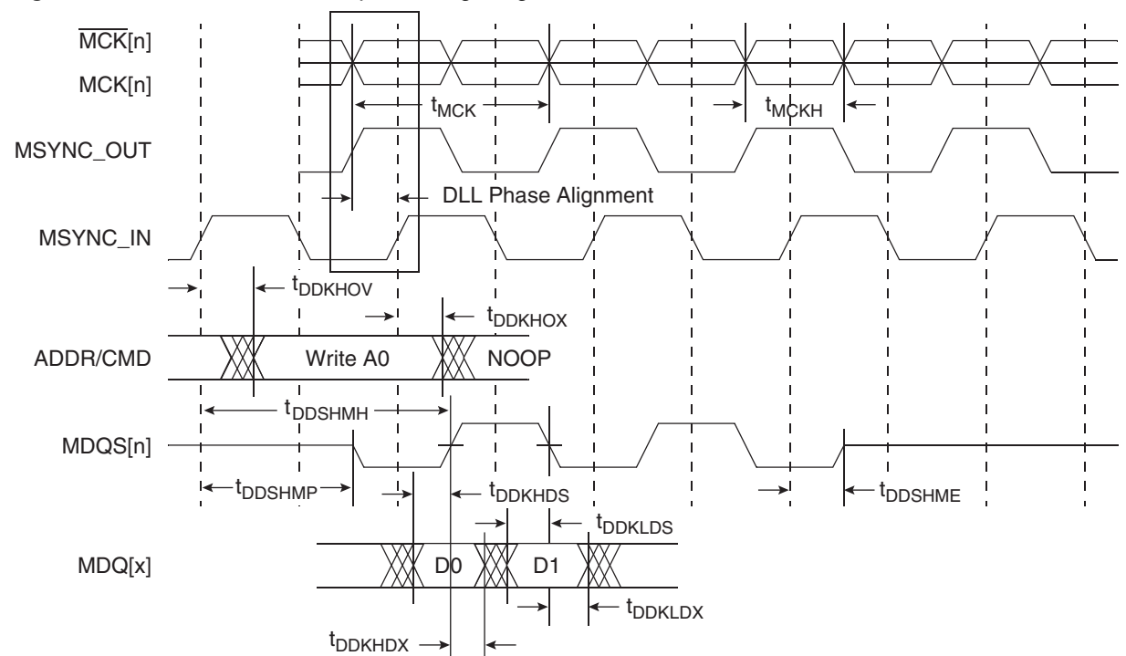
Figure 6-3. DDR SDRAM Output Timing Diagram
