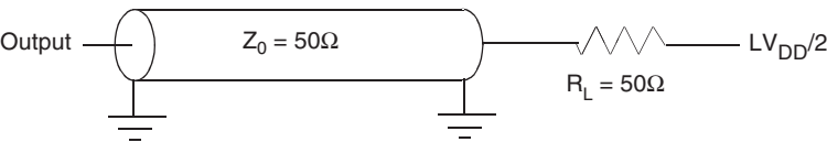
Figure 8-2. TSEC AC Test Load
