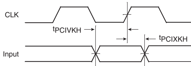
Figure 12-2. PCI-PCI-X Input AC Timing Measurement Conditions
