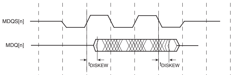
Figure 6-1. DDR SDRAM Interface Input Timing
