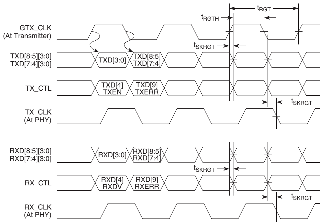
Figure 8-8. RGMII and RTBI AC Timing and Multiplexing Diagrams
