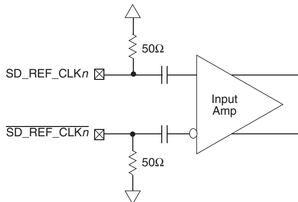
Figure 2-29. Receiver of SerDes Reference Clocks
