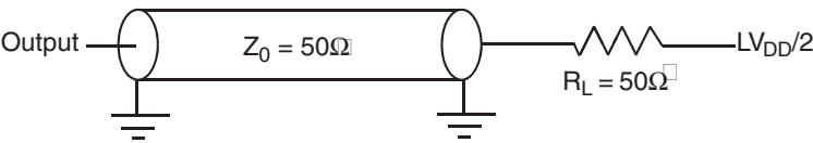
Figure 2-14. USB AC Test Load
