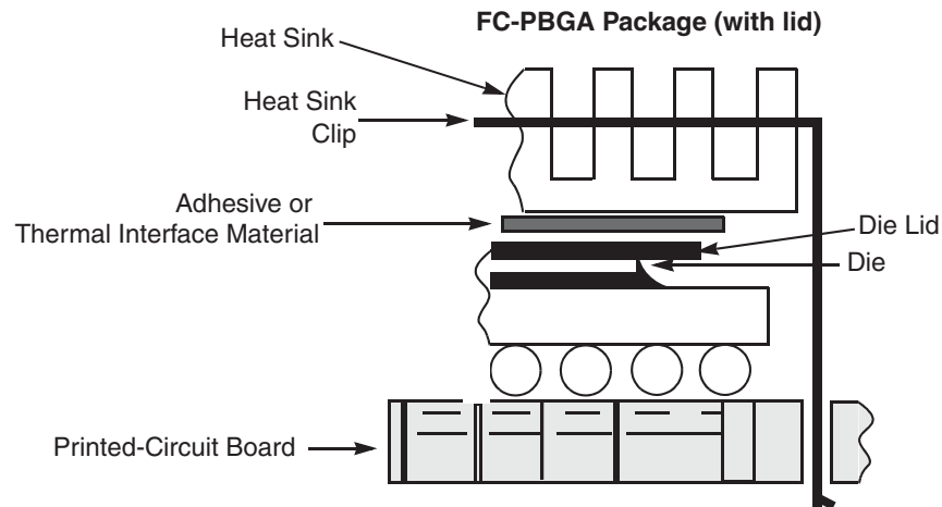
Figure 3-13. Package Exploded Cross-Sectional View.FC-PBGA (with Lid) Package
