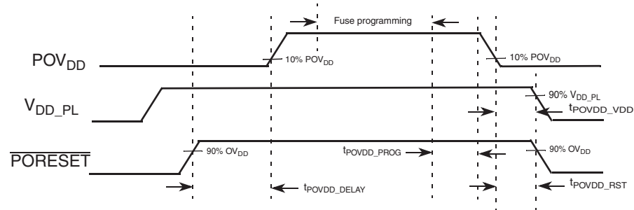
Figure 2-2. POV_{DD} Timing Diagram
