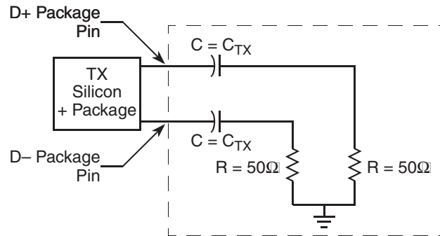
Figure 2-3. SGMII AC Test/Measurement Load
