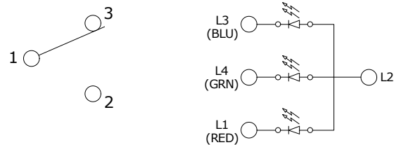
SWITCH SCHEMATIC (MOMENTARY)
