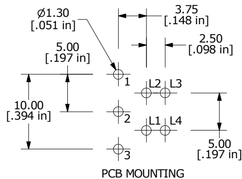
PCB MOUNTING
