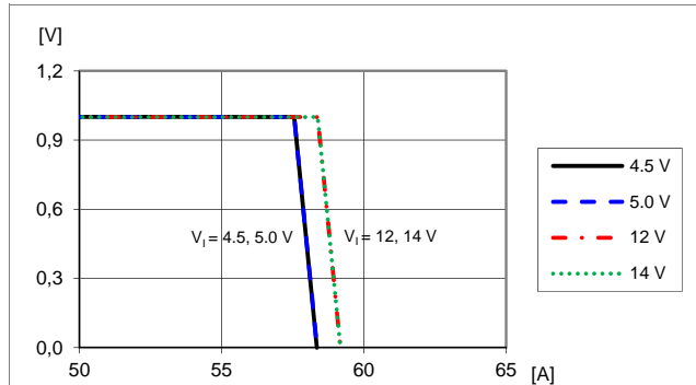
Output voltage vs. load current at T_{Pt} = +25 °C , V_O = 1.0 V . Note: Output enters hiccup mode at current limit.
