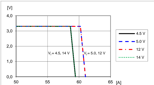
Output voltage vs. load current at T_{Pt} = +25 °C , V_O = 3.3 V . Note: Output enters hiccup mode at current limit.
