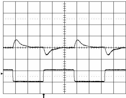
Output voltage response to load current step- change (5 - 15 - 5 A) at: T_{ref} = +25^{\circ}C , V_1 = 53 V , C_o = 2.2 mF
