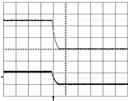
Shut-down enabled by disconnecting V_1 at: T_{ref} = +25^{\circ}C , V_1 = 53 V , I_O = 20 A resistive load.
