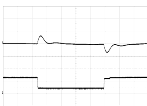
Output voltage response to load current step-change (8.75-26.25-8.75 A) at: T_{P1}, T_{P3} = +25^\circ\text{C}, V_I = 53\text{ V}, C_O = 3.5\text{ mF}. Top trace: output voltage (0.2 V/div.). Bottom trace: output current (20 A/div.). Time scale: (0.5 ms/div.).
