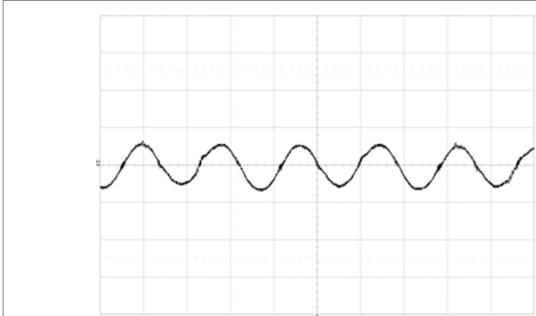
Output voltage ripple at: T_{P1}, T_{P3} = +25^\circ\text{C}, V_I = 53\text{ V}, I_O = 35\text{ A} resistive load. Trace: output voltage (50 mV/div.). Time scale: (2 \mu\text{s} /div.).
