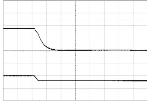
Shut-down enabled by disconnecting V_I at: T_{P1}, T_{P3} = +25^\circ\text{C}, V_I = 53\text{ V}, I_O = 35\text{ A} resistive load. Top trace: output voltage (5 V/div.). Bottom trace: input voltage (50 V/div.). Time scale: (2 ms/div.).
