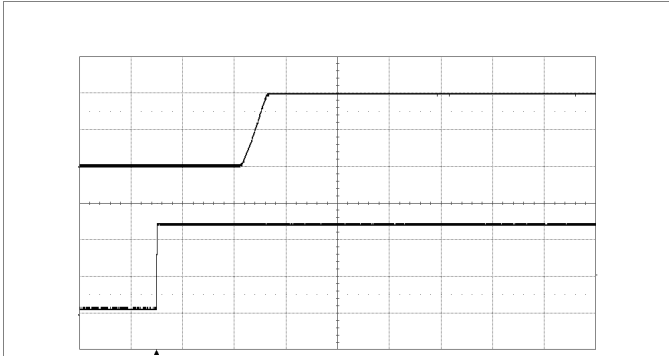
Start-up enabled by connecting V_I at: T_{P1} = +25^\circ\text{C} , V_I = 12\text{ V} , V_O = 1.0\text{ V} C_O = 470\ \mu\text{F}/10\ \text{m}\Omega , I_O = 40\ \text{A} Top trace: output voltage (0.5 V/div.). Bottom trace: input voltage (5 V/div.). Time scale: (20 ms/div.).
