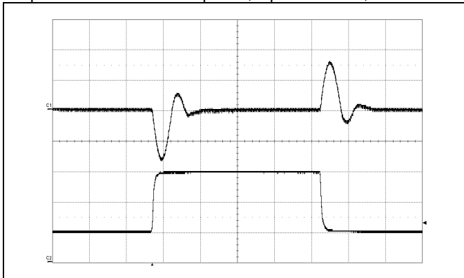
Output voltage response to load current step- Top trace: output voltage (200 mV/div.), change (10-30-10 A) at: Bottom trace: load current (10 A/div.). T_{P1} = +25^{\circ}\text{C} , V_I = 12\text{ V} , V_O = 1.0\text{ V} Time scale: (0.1 ms/div.). di/dt = 2\text{ A}/\mu\text{s} , f_{sw} = 320\text{ kHz} , C_O = 470\text{ }\mu\text{F}/10\text{ m}\Omega Optimized PID Control Loop and no NLR
