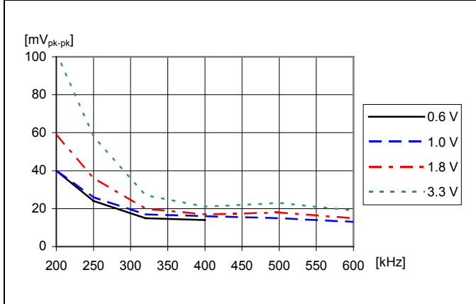
Output voltage ripple V_{pk-pk} at: T_{P1} = +25^{\circ}\text{C} , V_I = 12\text{ V} , C_O=470\text{ }\mu\text{F}/10\text{ m}\Omega , I_O = 40\text{ A} resistive load. Default configuration except changed frequency.
