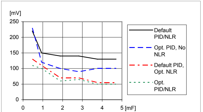
Load transient peak voltage deviation vs. external capacitance. Step-change (10-30-10 A). Parallel coupling of capacitors with 470 \mu F/10 m \Omega , T_{P1} = +25^\circ C. V_I=12 V, V_O=3.3 V, f_{sw}=320 kHz, di/dt=2 A/ \mu s
