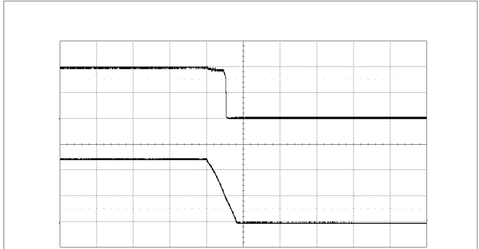
Shut-down enabled by disconnecting V_I at: T_{P1} = +25^\circ\text{C} , V_I = 12\text{ V} , V_O = 1.0\text{ V} C_O = 470\ \mu\text{F}/10\ \text{m}\Omega , I_O = 40\ \text{A} Top trace: output voltage (0.5 V/div.). Bottom trace: input voltage (5 V/div.). Time scale: (2 ms/div.).
