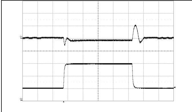
Output voltage response to load current step- Top trace: output voltage (200 mV/div.), change (10-30-10 A) at: Bottom trace: load current (10 A/div.). T_{P1} = +25^{\circ}\text{C} , V_I = 12\text{ V} , V_O = 1.0\text{ V} Time scale: (0.1 ms/div.). di/dt = 2\text{ A}/\mu\text{s} , f_{sw} = 320\text{ kHz} , C_O = 470\text{ }\mu\text{F}/10\text{ m}\Omega Default PID Control Loop and NLR
