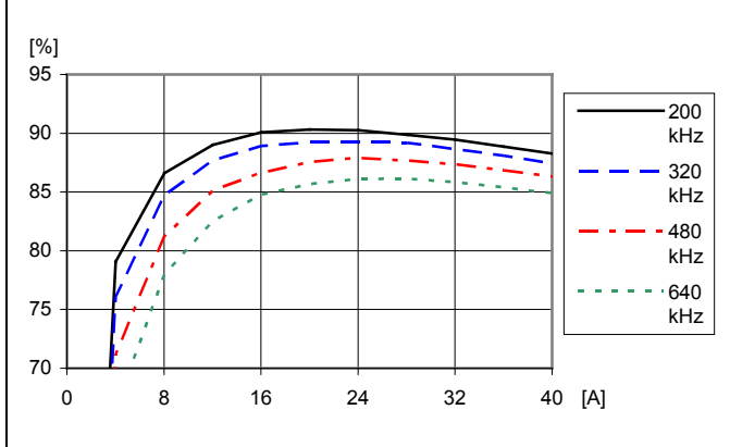
Efficiency vs. load current and switching frequency at T_{P1} = +25^{\circ}\text{C} , V_I=12\text{ V} , V_O=1.0\text{ V} , C_O=470\text{ }\mu\text{F}/10\text{ m}\Omega Default configuration except changed frequency
