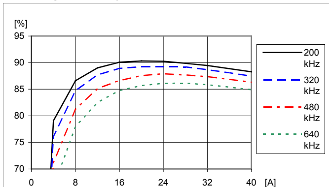
Efficiency vs. load current and switch frequency at T_{P1} = +25^\circ\text{C} , V_I=12\text{ V} , V_O=1.0\text{ V} , C_O=470\text{ }\mu\text{F}/10\text{ m}\Omega Default configuration except changed frequency
