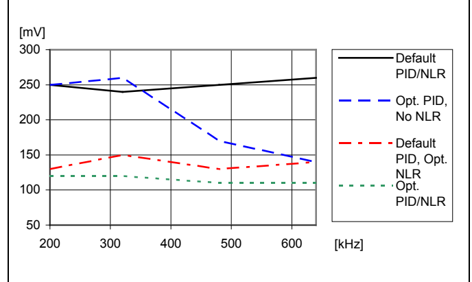
Load transient peak voltage deviation vs. frequency. Step-change (10-30-10 A). T_{P1} = +25^{\circ}\text{C} , V_I=12\text{ V} , V_O=1.0\text{ V} , C_O=470\text{ }\mu\text{F}/10\text{ m}\Omega
