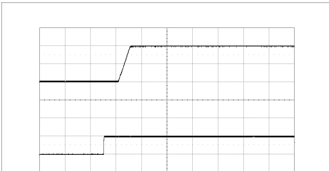
Start-up by enabling CTRL signal at: T_{P1} = +25^\circ\text{C} , V_I = 12\text{ V} , V_O = 1.0\text{ V} C_O = 470\ \mu\text{F}/10\ \text{m}\Omega , I_O = 40\ \text{A} Top trace: output voltage (0.5 V/div.). Bottom trace: CTRL signal (5 V/div.). Time scale: (20 ms/div.).
