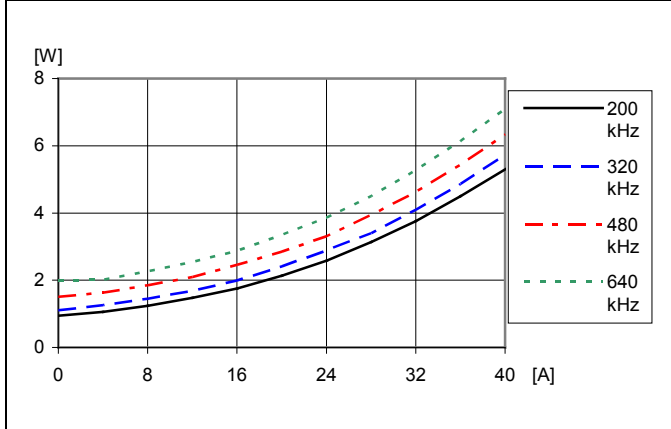
Dissipated power vs. load current and switching frequency at T_{P1} = +25^{\circ}\text{C} , V_I=12\text{ V} , V_O=1.0\text{ V} , C_O=470\text{ }\mu\text{F}/10\text{ m}\Omega Default configuration except changed frequency
