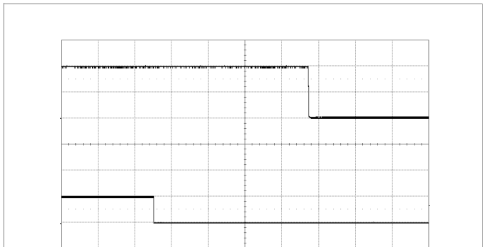
Shut-down enabled by disconnecting CTRL signal at: T_{P1} = +25^\circ\text{C} , V_I = 12\text{ V} , V_O = 1.0\text{ V} C_O = 470\ \mu\text{F}/10\ \text{m}\Omega , I_O = 40\ \text{A} Top trace: output voltage (0.5 V/div.). Bottom trace: CTRL signal (5 V/div.). Time scale: (2 ms/div.).
