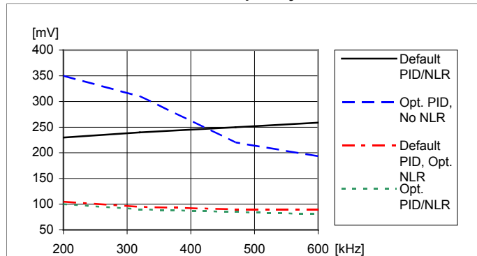
Load transient peak voltage deviation vs. frequency. Step-change (10-30-10 A). T_{P1} = +25^\circ C. V_I=12 V, V_O=1.0 V, C_O=470 \mu F/10 m \Omega
