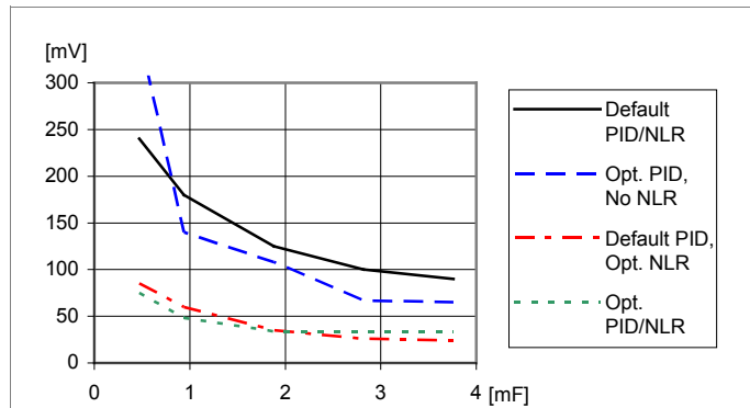
Load transient peak voltage deviation vs. external capacitance. Step-change (10-30-10 A). Parallel coupling of capacitors with 470 \mu F/10 m \Omega , T_{P1} = +25^\circ C. V_I=12 V, V_O=1.0 V, f_{sw}=320 kHz, di/dt=2 A/ \mu s
