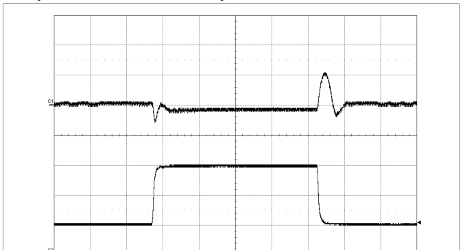
Output voltage response to load current step-change (10-30-10 A) at: T_{P1} = +25^\circ C, V_I = 12 V, V_O = 1.0 V, di/dt=2 A/ \mu s, f_{sw}=320 kHz, C_O=470 \mu F/10 m \Omega
