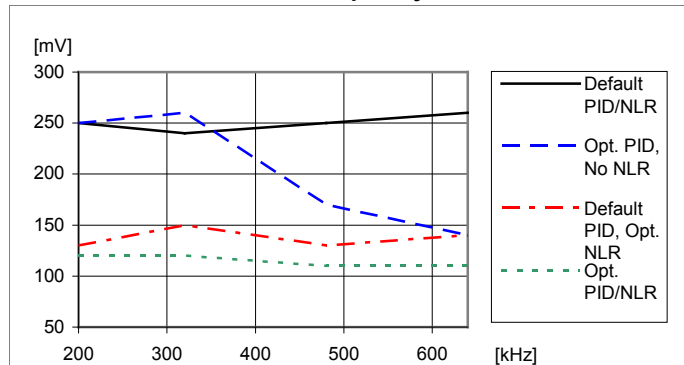
Load transient peak voltage deviation vs. frequency. Step-change (10-30-10 A). T_{P1} = +25^\circ C. V_I=12 V, V_O=1.0 V, C_O=470 \mu F/10 m \Omega
