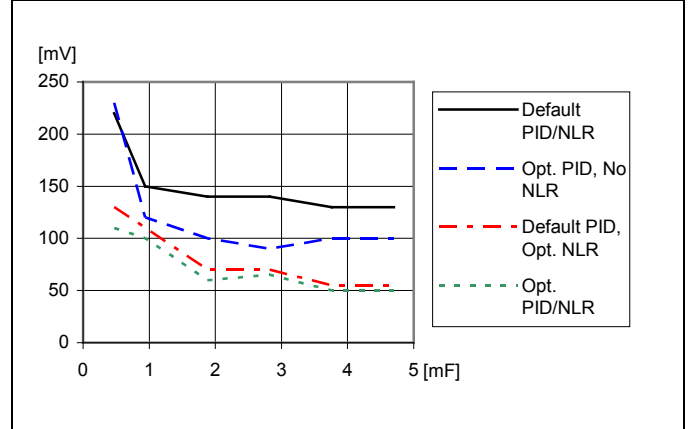
Load transient peak voltage deviation vs. decoupling capacitance. Step-change (10-30-10 A). Parallel coupling of capacitors with 470\text{ }\mu\text{F}/10\text{ m}\Omega , T_{P1} = +25^{\circ}\text{C} , V_I=12\text{ V} , V_O=3.3\text{ V} , f_{sw}=320\text{ kHz} , di/dt=2\text{ A}/\mu\text{s}
