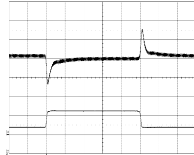
Output voltage response to load current step- change (3.75-11.25-3.75 A) at: T_{ref} = +25^{\circ}\text{C} , V_i = 53\text{ V} . Top trace: output voltage (200 mV/div.). Bottom trace: load current (10 A/div.). Time scale: (0.1 ms/div.).
