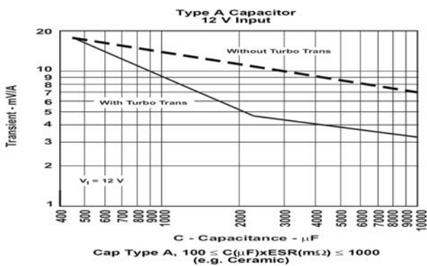
TurboTrans C 0 Values & Required R TT Selection Table
