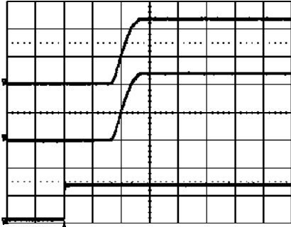
Start-up enabled by connecting V_i at: T_{ref} = +25^\circ\text{C} , V_i = 27\text{ V} , I_{o1} = 0.62\text{ A} , I_{o2} = 0.62\text{ A} resistive load. Top trace: output voltage 1 (5.0 V/div.). Mid trace: output voltage 2 (5.0 V/div.). Bottom trace: input voltage (20 V/div.). Time scale: (2 ms/div.).
