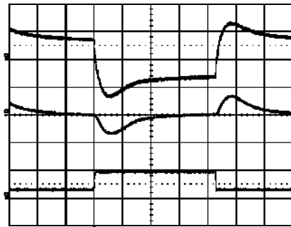
Output voltage response to load current step-change, output 1 (0.16-0.47-0.16 A) at: T_{ref} = +25^\circ\text{C} , V_i = 27\text{ V} , I_{o2} = 0.62\text{ A} . Top trace: output voltage 2 (100 mV/div.). Mid trace: output voltage 1 (100 mV/div.). Bottom trace: load current (0.5 A/div.). Time scale: (0.1 ms/div.).
