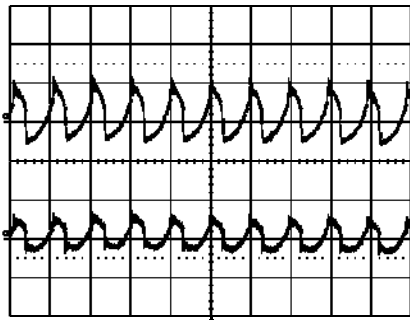
Output voltage ripple at: T_{ref} = +25^\circ\text{C} , V_i = 27\text{ V} , I_{o1} = 0.62\text{ A} , I_{o2} = 0.62\text{ A} resistive load. Top trace: output voltage 1 (5 mV/div.). Bottom trace: output voltage 2 (5 mV/div.). Time scale: (2 \mu\text{s} /div.).
