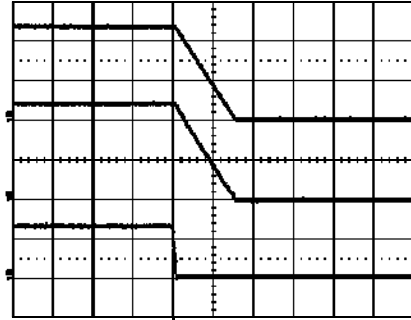
Shut-down enabled by disconnecting V_i at: T_{ref} = +25^\circ\text{C} , V_i = 27\text{ V} , I_{o1} = 0.62\text{ A} , I_{o2} = 0.62\text{ A} resistive load. Top trace: output voltage 1 (5.0 V/div.). Mid trace: output voltage 2 (5.0 V/div.). Bottom trace: input voltage (20 V/div.). Time scale: (0.5 ms/div.).
