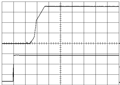
Start-up enabled by connecting V_i at: T_{ref} = +25^{\circ}\text{C} , V_i = 53\text{ V} , I_o = 5\text{ A} resistive load. Top trace: output voltage (0.5 V/div.). Bottom trace: input voltage (20 V/div.). Time scale: (2 ms/div.).
