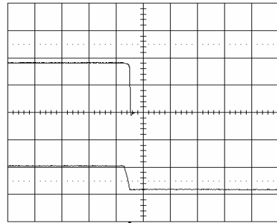
Shut-down enabled by disconnecting V_i at: T_{ref} = +25^{\circ}\text{C} , V_i = 53\text{ V} , I_o = 5\text{ A} resistive load. Top trace: output voltage (1.0 V/div.). Bottom trace: input voltage (50 V/div.). Time scale: (1 ms/div.).
