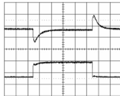
Output voltage response to load current step-change (1.25-3.75-1.25 A) at: T_{ref} = +25^{\circ}\text{C} , V_i = 53\text{ V} . Top trace: output voltage (200 mV/div.). Bottom trace: load current (2 A/div.). Time scale: (0.1 ms/div.).
