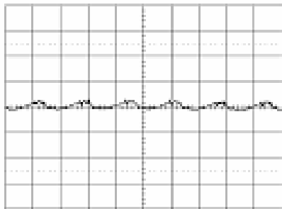
Output voltage ripple at: T_{ref} = +25^{\circ}\text{C} , V_i = 53\text{ V} , I_o = 5\text{ A} resistive load. Trace: output voltage (20 mV/div.). Time scale: (2 \mu\text{s} /div.).
