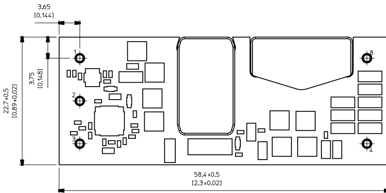
RECOMMENDED FOOTPRINT - TOP VIEW
