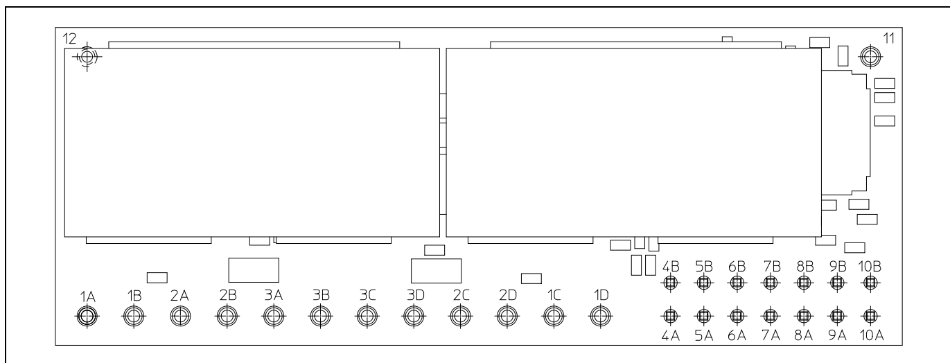
Pin layout, top view (component placement for illustration only).
