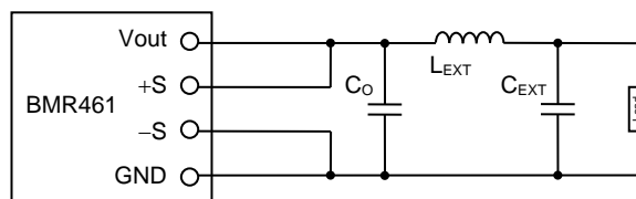
External output filter with inductor (pi filter).
