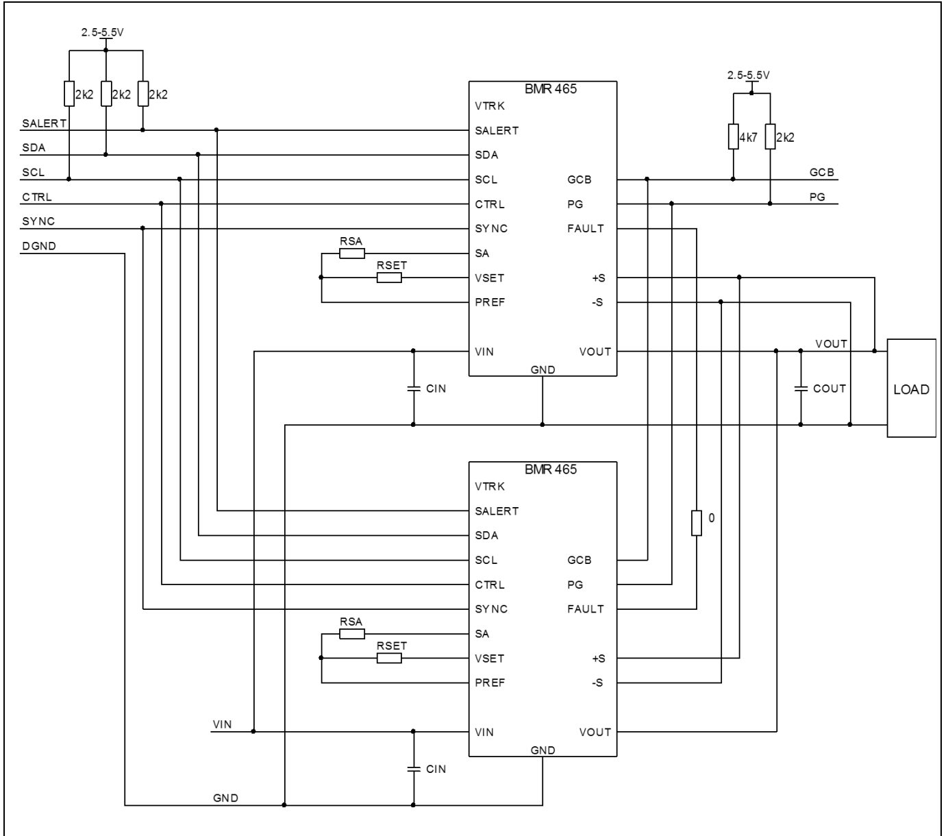
Parallel operation.
