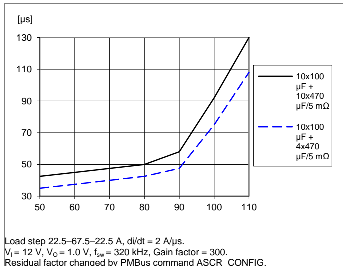
Recovery time vs. control loop residual setting and output capacitance.
