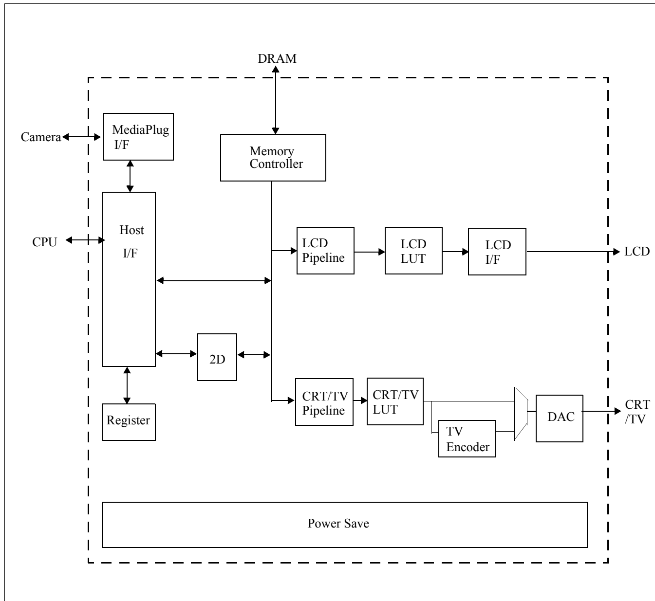
Figure 4-1: S1D13506 Block Diagram
