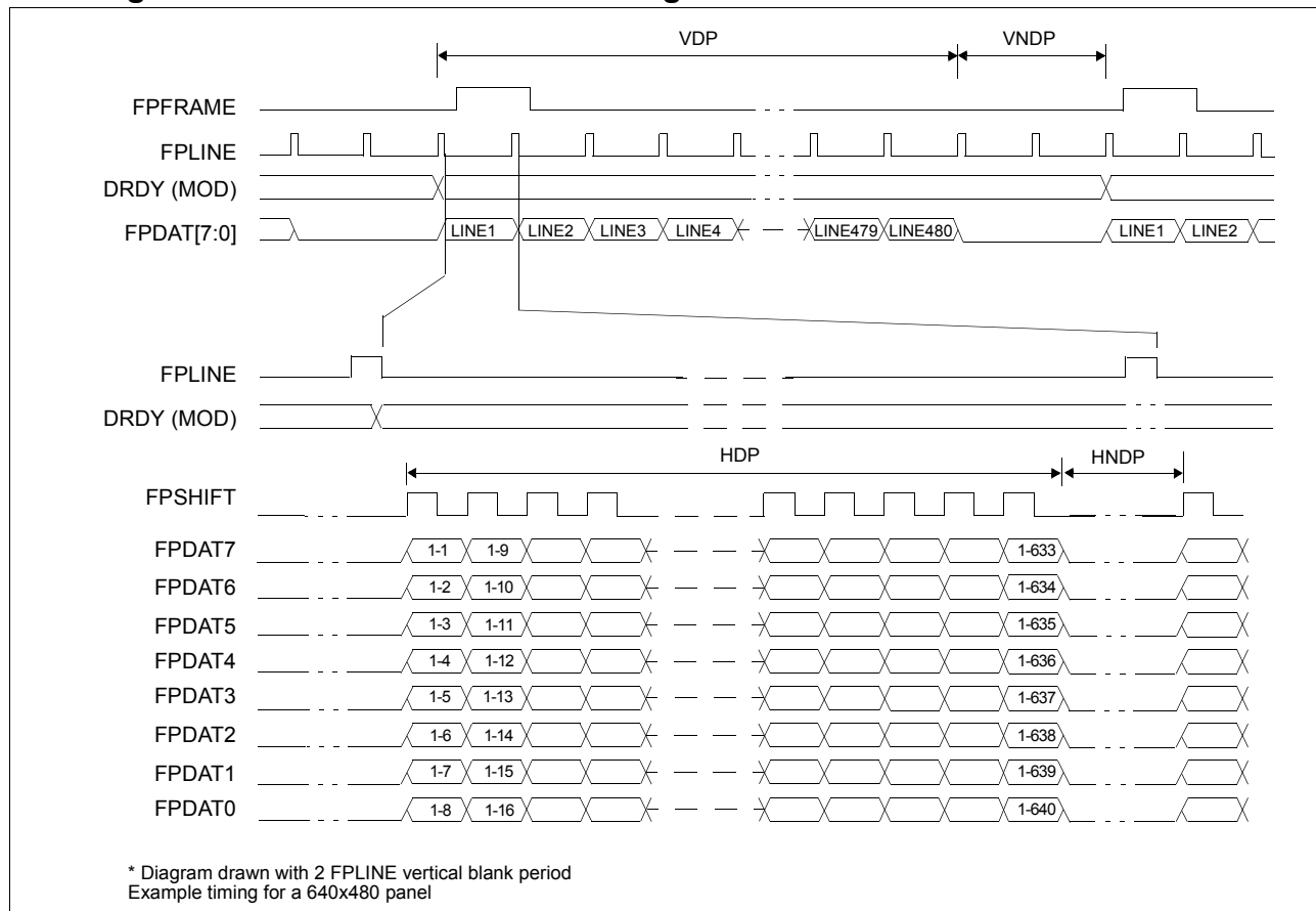
Figure 7-24: Single Monochrome 8-Bit Panel Timing
