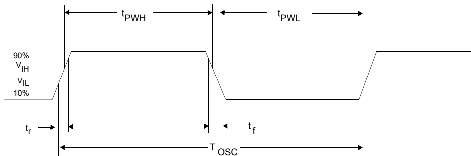
Figure 7-11: CLKI Clock Input Requirements
