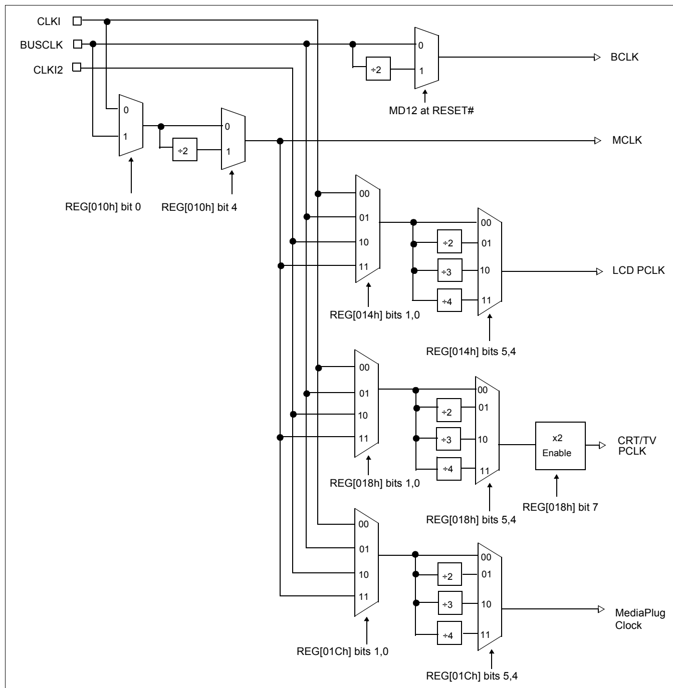
Figure 20-1: Clock Selection
