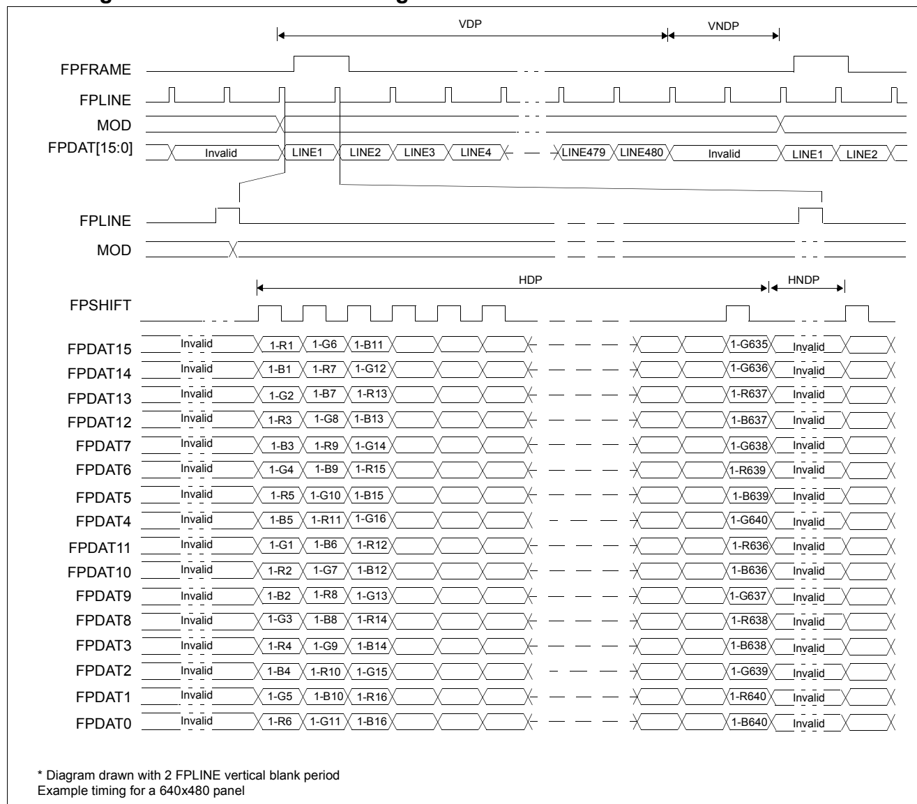
Figure 7-32: Single Color 16-Bit Panel Timing
