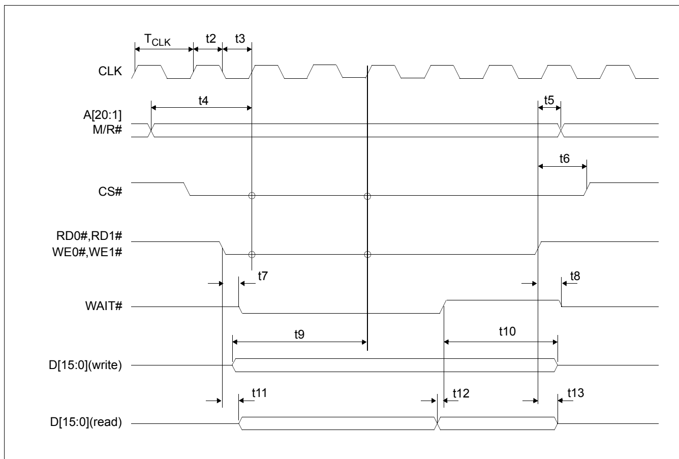
Figure 7-1: Generic Timing
