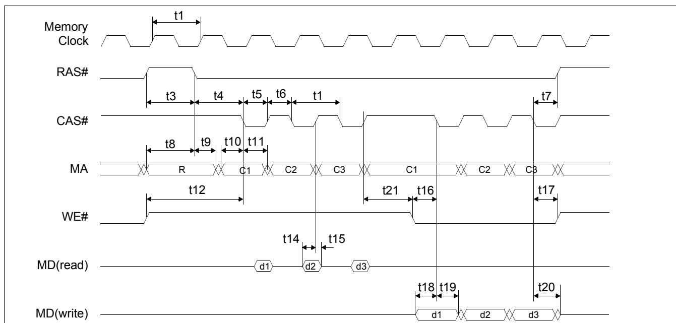
Figure 7-17: FPM-DRAM Read-Write Timing
