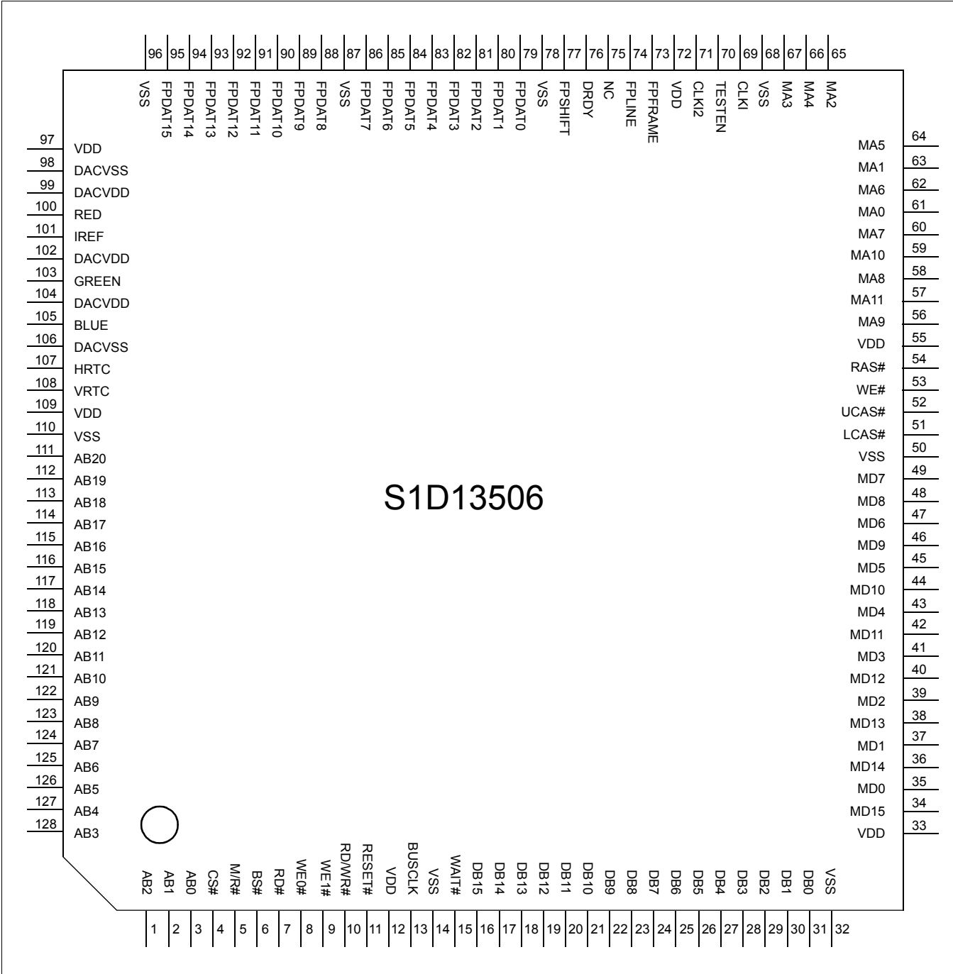
Figure 5-1: Pinout Diagram
