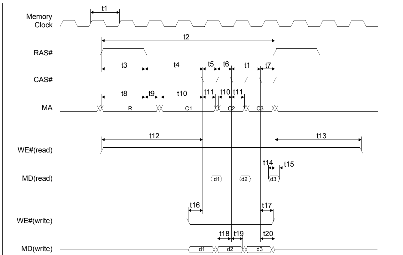
Figure 7-16: FPM-DRAM Page Mode Timing
