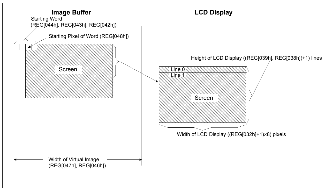
Figure 11-2: Image Manipulation
