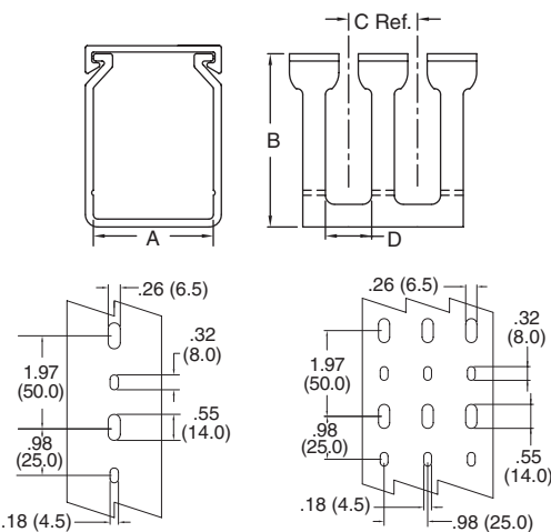
Mounting Style 1
