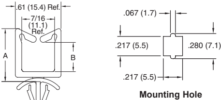
Mounting Hole
