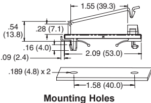
Mounting Holes
