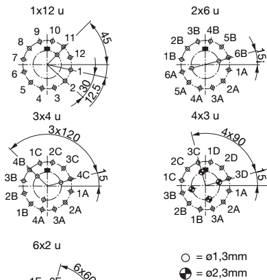
Drilling diagram for indexing angle 30°
