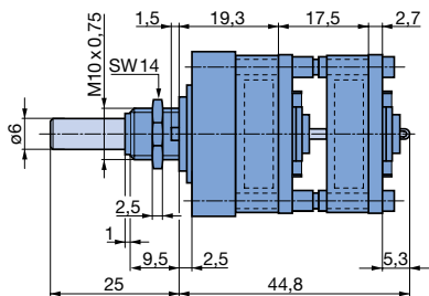
Drilling diagram for indexing angle 15°
