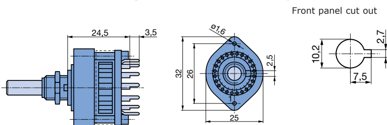
Drilling diagram for indexing angle 30°
