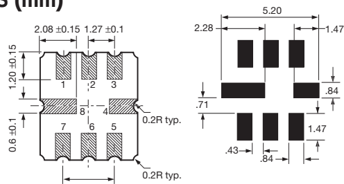
Figure 2) DSF-400 Suggested Land Pattern
