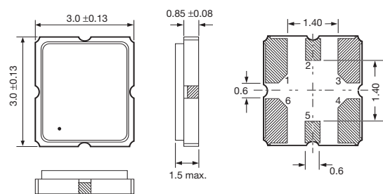
Figure 3) DSF947.5 Top, Side, Bottom and End views
