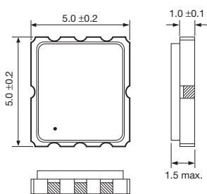
Figure 1) DSF400 Top, Side, Bottom and End views
