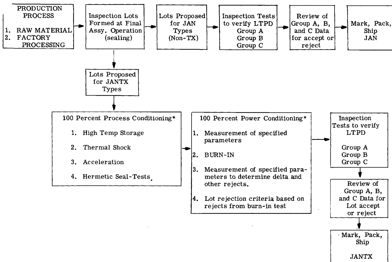
*ORDER OF THE TESTS IN THE BLOCKS SHALL BE PERFORMED AS SHOWN FIGURE 2. Order of procedure diagram for JAN (Non-TX) and JANTX types.
