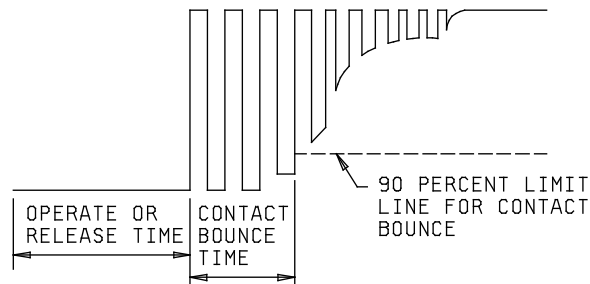
FIGURE 6. Typical circuit for operate and release time, contact bounce and contact stabilization time with typical traces.
