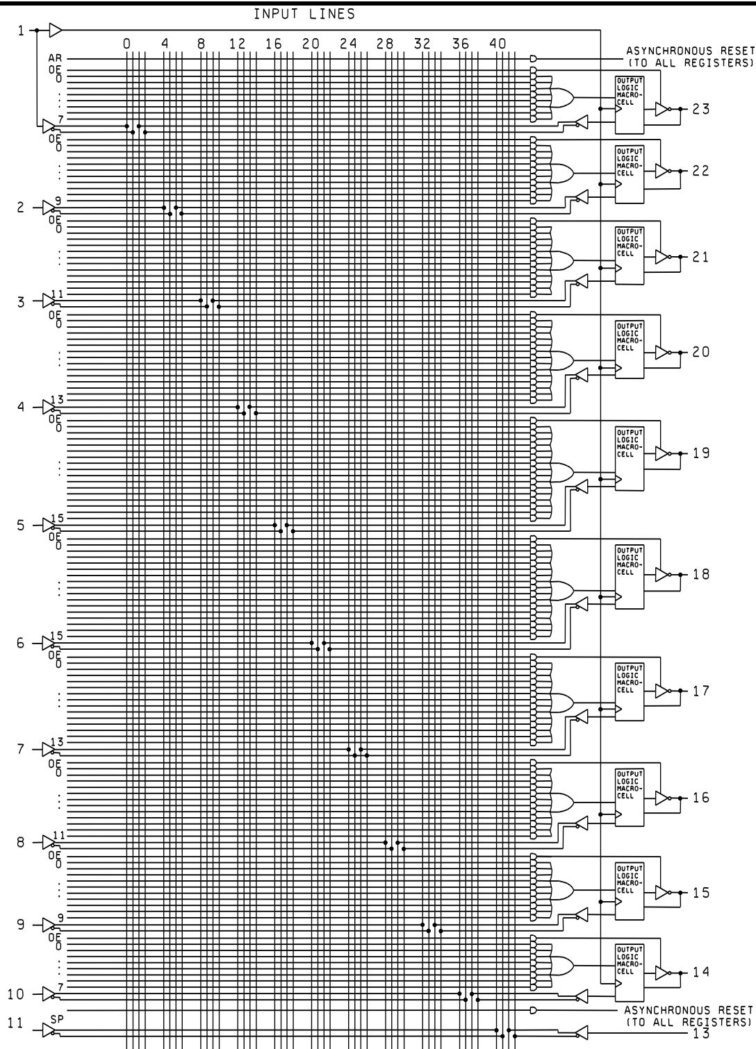
FIGURE 3. Logic diagram (unprogrammed).
