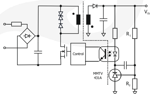
Fig. 5 Secondary side regulation of a flyback converter
