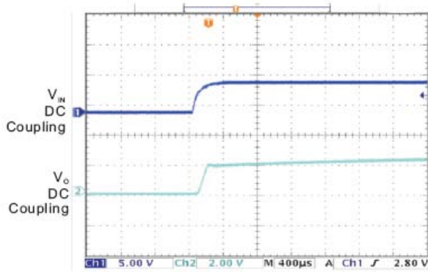
13. Turn-on Response
