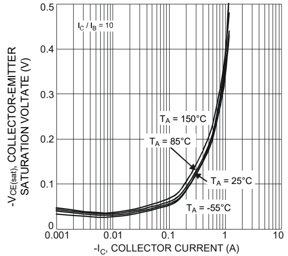
Fig.9 V_{CE(sat)} v I_C
