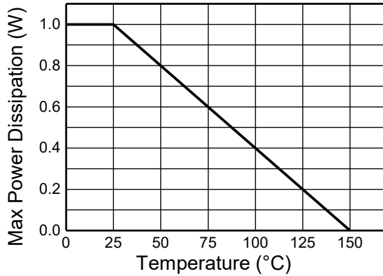
Fig.1 Derating Curve
