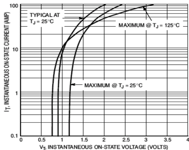
Figure 7. On-State Characteristics
