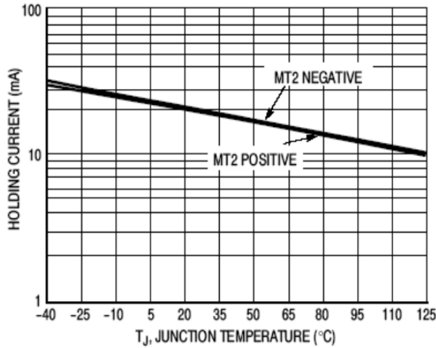
Figure 3. Typical Holding Current versus Junction Temperature
