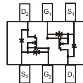
Equivalent Circuit
