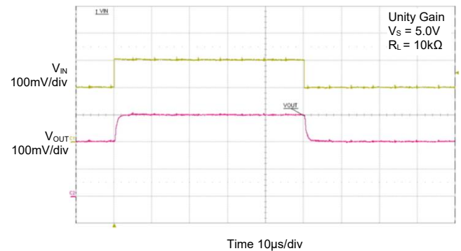
Small-Signal Response
