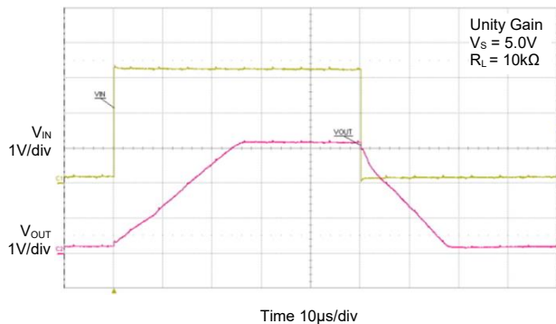
Large-Signal Response
