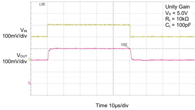
Small-Signal Response
