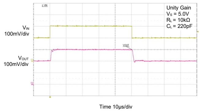
Small-Signal Response
