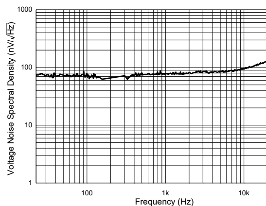
Figure 2. Input Voltage Noise in Zero-Drift Amplifier (AS2333)
