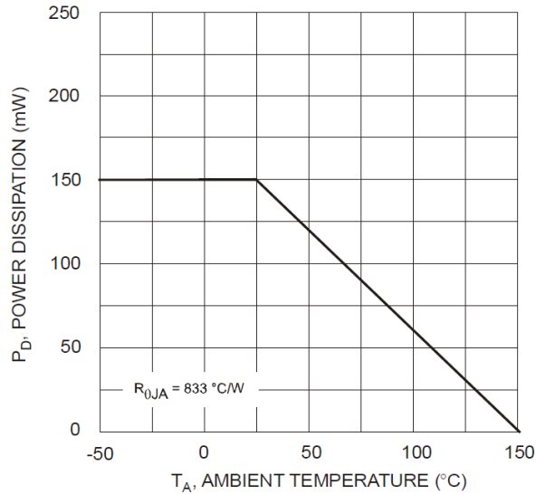
Figure 1. Derating Curve
