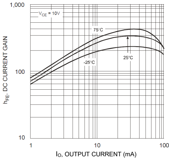
Figure 3. h_{FE} vs. I_O
