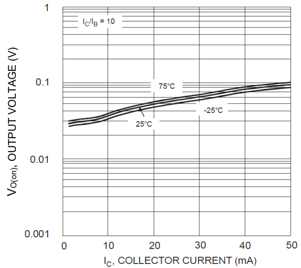
Figure 2. V_{O(on)} vs. I_C
