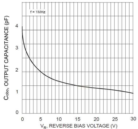
Figure 4. C_{obo} vs. V_R
