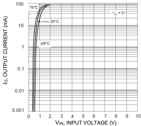
Figure 5. I_O vs. V_{IN}
