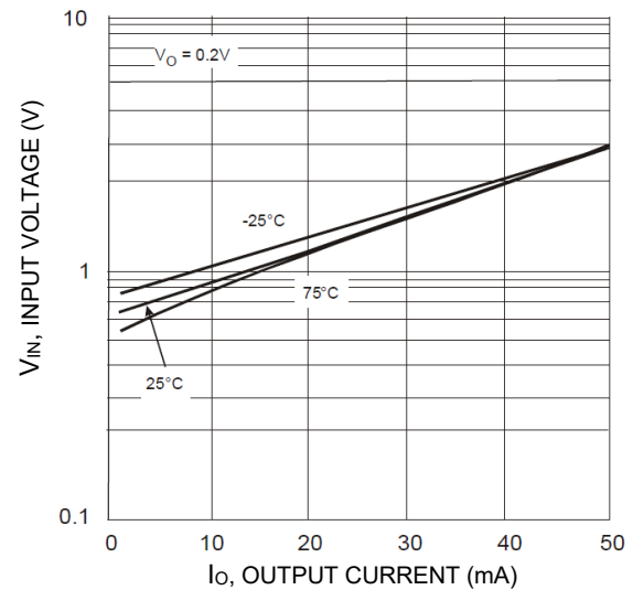
Figure 6. V_{IN} vs. I_O
