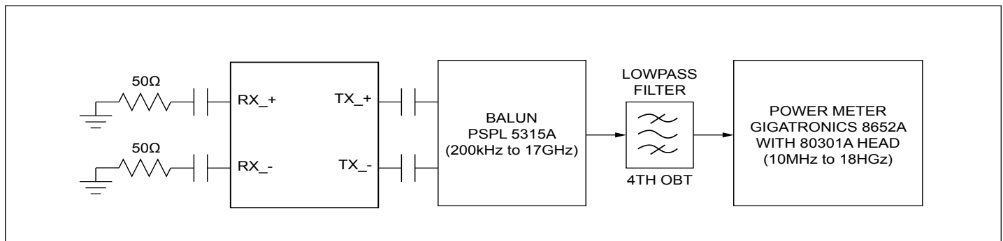
Figure 2. Noise Test Configuration
