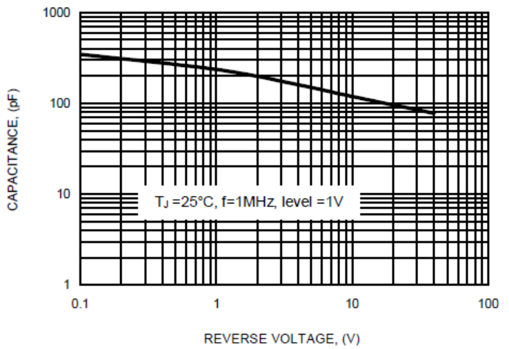
FIG.4-TYPICAL JUNCTION CAPACITANCE
