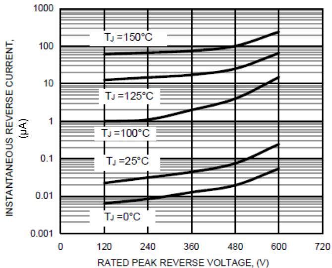
FIG.5-TYPICAL REVERSE CHARACTERISTICS
