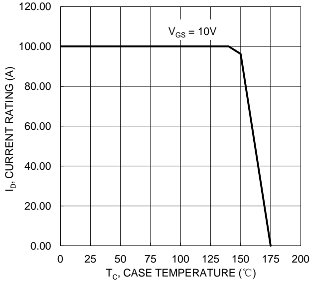
Figure 13. Current De-rating
